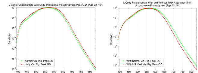
Fig 3: L- cone fundamentals with normal and modified visual pigment absorption function, as described in case (iii) [left] and case (iv) [right]
