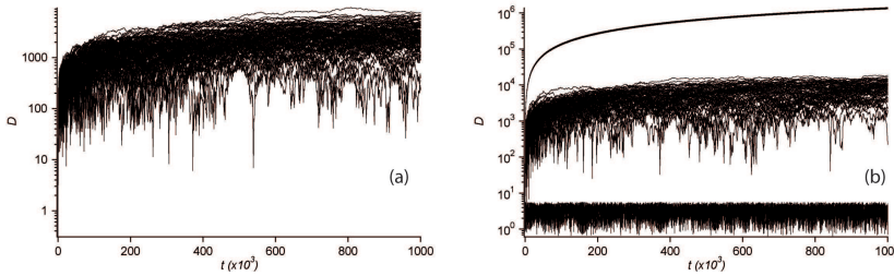
Figure 5. Distance covered by 100 atoms as a function of time. In (a), U_+ and E = 2.66 . In (b), U_- and E = 1.07 .
