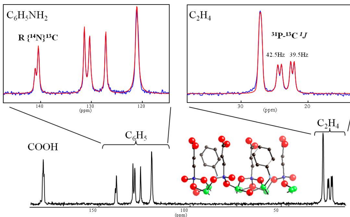
Figure 2 : ^{13}\text{C} CP-MAS spectrum (300 MHz, 14 kHz) of the crystalline layered phosphonate (\text{ZnO}_3\text{P C}_2\text{H}_4 \text{ CO}_2\text{H} - 0.5 \text{ C}_6\text{H}_5\text{NH}_2) [18] acquired with an accurate setting ( \pm 0.01^\circ ) of the MAS angle and optimized proton decoupling, which allows evidencing the ^{31}\text{P} - ^{13}\text{C} ^1J splitting on the first carbon of the aliphatic chain and the splitting of the ^{13}\text{C} - ^{14}\text{N} resonance by the dipolar/quadrupolar cross term ( \text{R}\{^{14}\text{N}\}^{13}\text{C} ).
