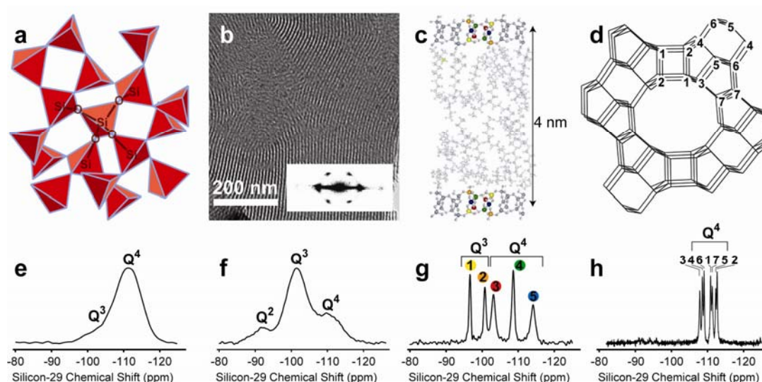
Figure 1 : (a) Schematic representation of an amorphous \text{SiO}_2 structure, with \text{SiO}_4 tetrahedra shown in red, and (e) ^{29}\text{Si} spin-echo MAS NMR spectrum of commercial silica with 99% enrichment in ^{29}\text{Si} . (b) Transmission-electron microscopy (TEM) image and electron diffraction pattern (inset) and (f) ^{29}\text{Si}\{^1\text{H}\} CPMAS NMR spectrum of an hexagonal mesoporous silica composite.[4] (c) In-plane view of a layered silicate-surfactant mesophase consisting of thin (0.8 nm) molecularly-ordered silicate sheets with five distinct (colored) Si atom sites giving rise to five narrow ^{29}\text{Si} resonances in the corresponding ^{29}\text{Si}\{^1\text{H}\} CPMAS NMR spectrum (g), and separated by alkylammonium surfactant species.[5] (d) Schematic representation of the highly ordered silicate framework structure and (h) ^{29}\text{Si} MAS NMR spectrum with extremely narrow resonances of zeolite ZSM-12 (courtesy D.H. Brouwer).
