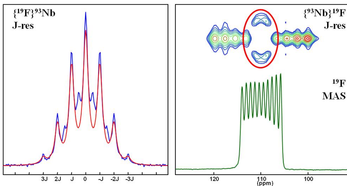
Figure 6 : Central transition selective \{^{19}\text{F}\}^{93}\text{Nb} J -resolved experiment and its model with a 7 fold multiplet – 1D MAS spectrum, \delta_{\text{F}} = 110.1 ppm, ^1J = 344 Hz showing coupling to the 10 spin states of a single ^{93}\text{Nb} nucleus and \{^{93}\text{Nb}\}^{19}\text{F} J -resolved experiment showing that only the two center bands corresponding to \langle \pm 1/2 \rangle central transition of ^{93}\text{Nb} is manipulated during the ^{93}\text{Nb} excitation.
