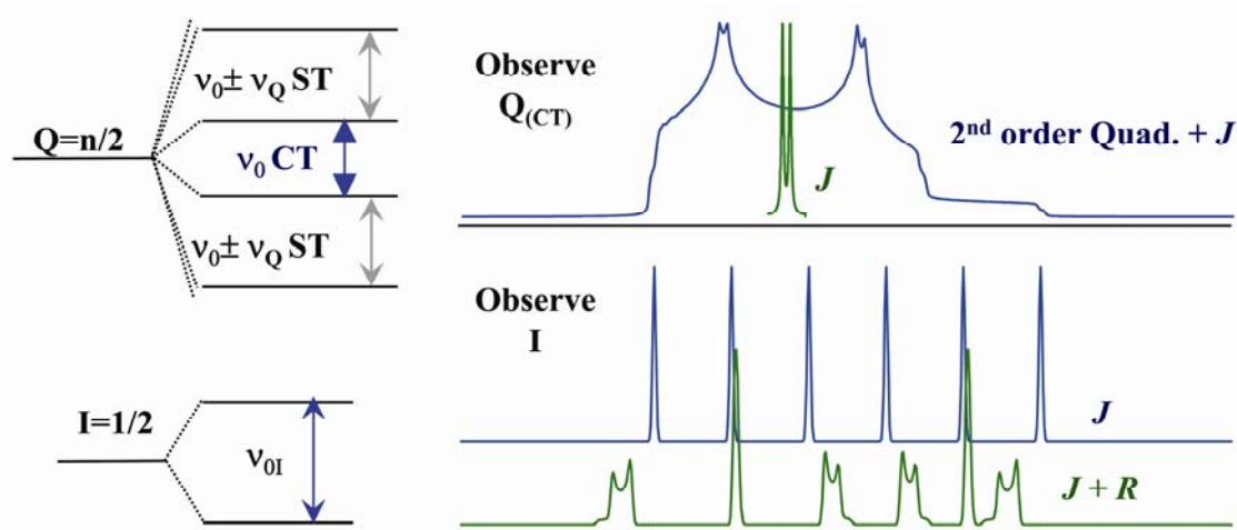
Figure 4 : Schematic representation of the effect of the J coupling between a quadrupolar nucleus Q ( I=5/2 ) and a dipolar nucleus I ( I=1/2 ). The central transition of the quadrupolar nucleus Q (top, in blue) is broadened to second order by the quadrupolar interaction and split in two by the J coupling to I (in green). The second order quadrupolar broadening can be removed in an MQMAS experiment allowing to only observe the J -coupling multiplet [76]. The signal of the I nucleus is split in a 2Q+1 (e.g., 6 for I=5/2 ) multiplet. Additional second order broadenings and shifts arise when R (the Dipolar Quadrupolar cross term) becomes significant.
