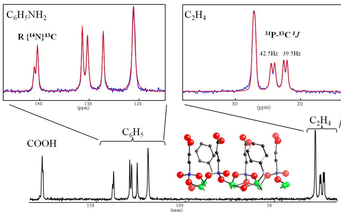
Figure 2 : ^{13}\text{C} CP-MAS spectrum (300 MHz, 14 kHz) of the crystalline layered phosphonate (\text{ZnO}_3\text{P C}_2\text{H}_4 \text{ CO}_2\text{H} - 0.5 \text{ C}_6\text{H}_5\text{NH}_2) [18] acquired with an accurate setting ( \pm 0.01^\circ ) of the MAS angle and optimized proton decoupling, which allows evidencing the ^{31}\text{P} - ^{13}\text{C} ^1J splitting on the first carbon of the aliphatic chain and the splitting of the ^{13}\text{C} - ^{14}\text{N} resonance by the dipolar/quadrupolar cross term ( \text{R}\{^{14}\text{N}\}^{13}\text{C} ).
