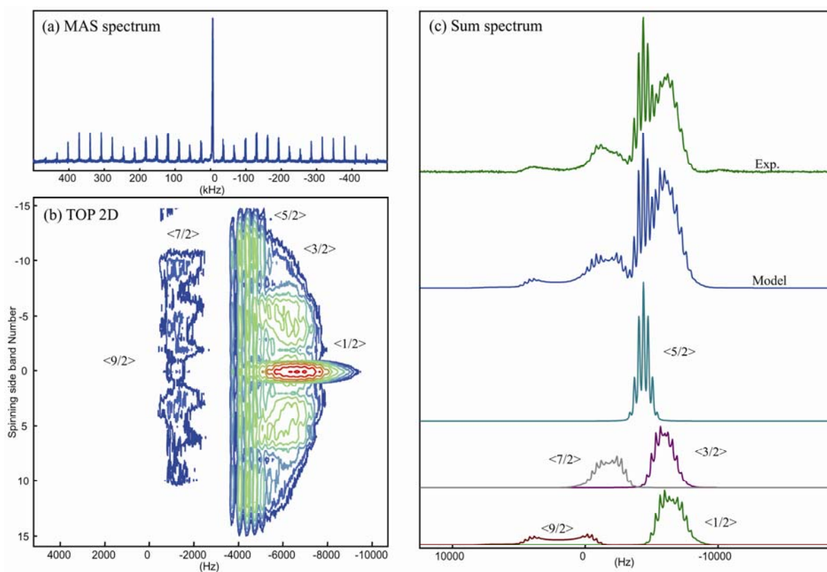
Figure 5 : TOP processing of the ^{93}\text{Nb} MAS spectrum of \text{CsNbF}_6 , \delta_{\text{Nb}} = -1580 ppm, C_Q = 10.2 MHz, \eta_Q = 0.45 (a) allowing 2D reconstruction of the TOP spectrum (b) and the computation of the infinite spinning rate TOP spectrum. The TOP spectrum can be modeled (c) considering a ^1J coupling of 344 Hz to 6 chemically bound cristallographically equivalent fluorine, which is reflected by the splitting of each observed transition of the ^{93}\text{Nb} resonance in a septuplet.
