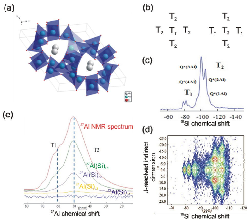
Figure 8 : (a) \alpha -Cordierite XRD structure[85], (b) connectivity of T_1 and T_2 sites, (c) ^{29}\text{Si} MAS NMR and (d) ^{29}\text{Si} J -Resolved spectra of 99% ^{29}\text{Si} -enriched cordierite featuring the ^2J(^{29}\text{Si-O-}^{29}\text{Si}) multiplets in the indirect dimension, (e) spectral editing of ^{27}\text{Al} NMR spectra in 99% ^{29}\text{Si} -enriched \alpha -cordierite, corresponding to the 1D spectrum (in red), and the contributions of \text{Al}(\text{OSi})_{\geq 1} (red), \text{Al}(\text{OSi})_{\geq 2} (purple), \text{Al}(\text{OSi})_{\geq 3} (yellow) and \text{Al}(\text{OSi})_{\geq 4} (blue) motives.
