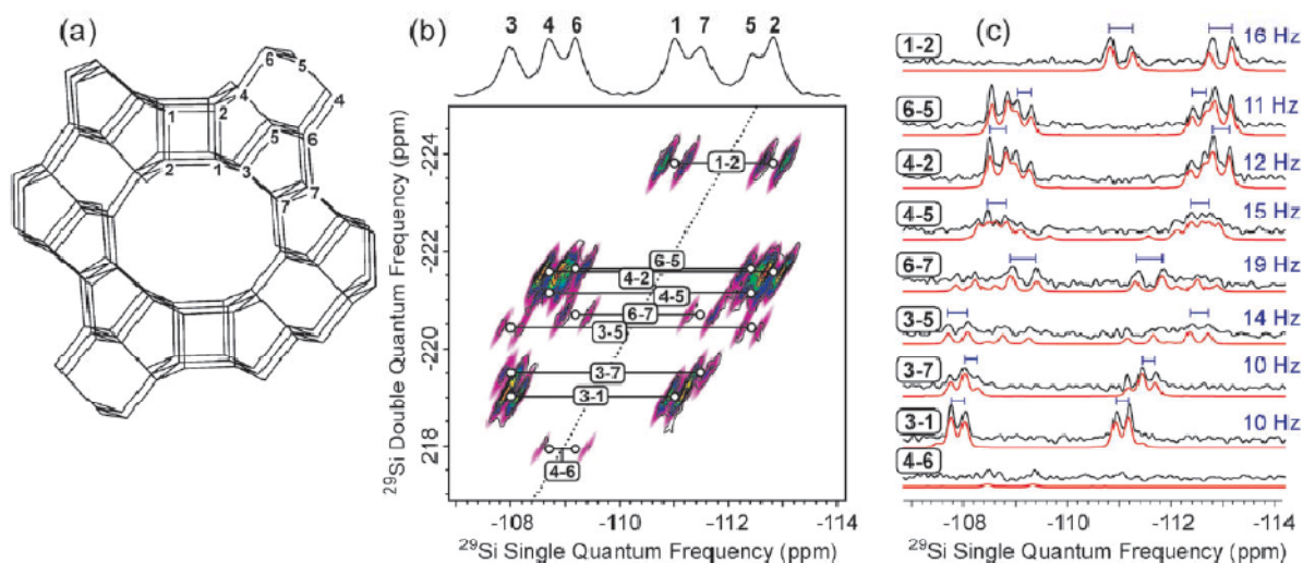
Figure 10 : (a) Schematic representation of the structure of ZSM-12. (b) Solid-state 2D refocused-INADEQUATE ^{29}\text{Si}\{^{29}\text{Si}\} NMR spectrum of siliceous zeolite ZSM-12 at natural abundance (black contour plots) and 2D spectral deconvolution (colored map) from which ^2J(^{29}\text{Si}-\text{O}-^{29}\text{Si}) values were extracted. (c) 1D ^{29}\text{Si} NMR slices extracted from the experimental spectrum (in black) and from the 2D deconvolution (in red), along with the measured J couplings [adapted from ref. 42].
