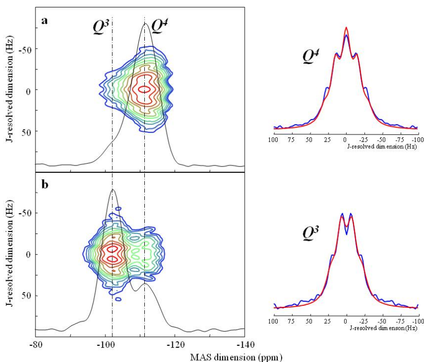
Figure 9 : J -resolved experiments performed on a ^{29}\text{Si} enriched \text{SiO}_2 sample « from the bottle » with (a) direct detection and (b) cross-polarization from ^1\text{H} . One-dimensional spectra superimposed to the 2D-lineshapes are projection onto the MAS dimension. The slices taken at along the J -resolved dimension at the peak maxima show a quadruplet for Q^3 and a quintuplet for Q^4 tentatively modeled with J -couplings of J(Q^3) \sim 14.0 Hz and J(Q^4) \sim 16.5 Hz.
