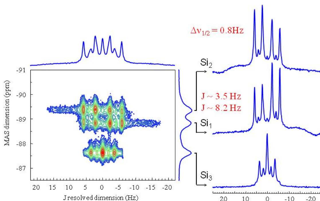
Figure 3 : J -resolved experiment on the crystalline Wollastonite \text{Ca}^{29}\text{SiO}_3 revealing ^2J(^{29}\text{Si} -O- ^{29}\text{Si}) couplings of a few hertz. The full J -resolved spectra can be perfectly modeled by considering ^{29}\text{Si} isotopic enrichment and strong coupling effects due to small chemical shift differences[adapted from ref 22]
