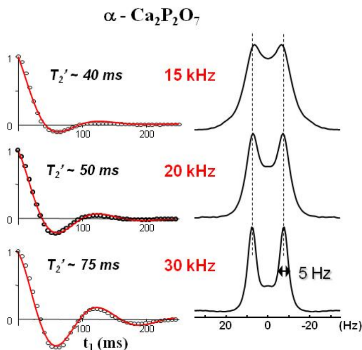
Figure 7. {}^{31}\text{P} J resolved MAS Spectra (7.0 T) of \alpha\text{-Ca}_2\text{P}_2\text{O}_7 acquired at exact Magic Angle ( \sim\pm 0.01^\circ ) showing the increased resolution of the {}^2J({}^{31}\text{P-O-}{}^{31}\text{P}) coupling with increasing MAS rate, allowing improved removal of residual contributions to transverse dephasing.
