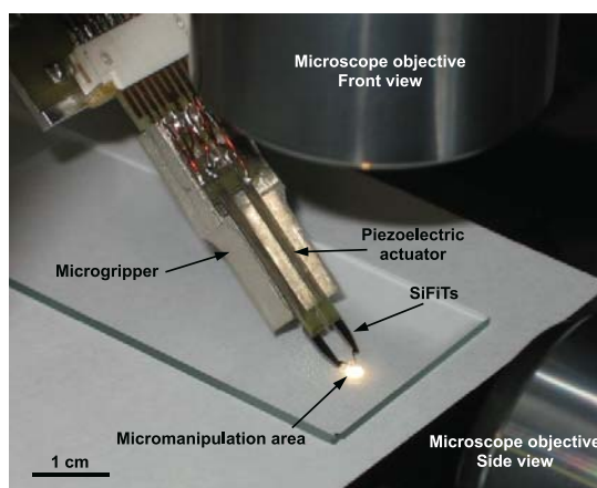
Fig. 6. Close view of the micromanipulation station
