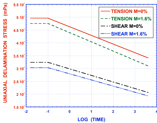
Fig. 3. Delamination stresses [4]
