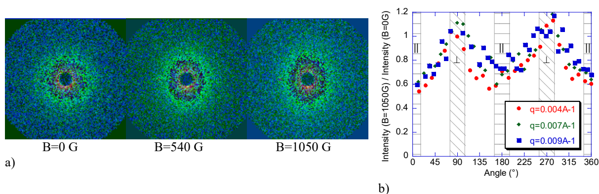
Figure 5: Deformation of hollow magnetic shells (system B \perp eq ) studied by anisotropic SANS.
