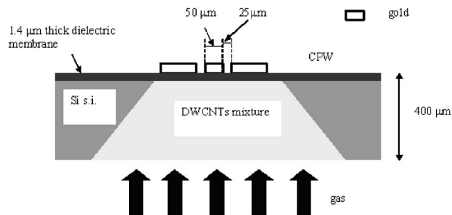
FIG. 1. Millimeterwave gas sensor based on carbon nanotubes.
