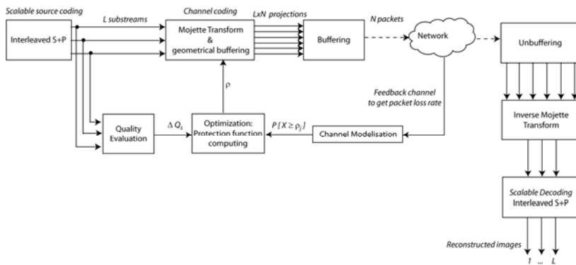
Fig. 8: General joint LAR-Mojette coding scheme
