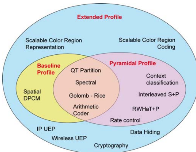
Fig. 1: Specific coding parts for LAR profiles
