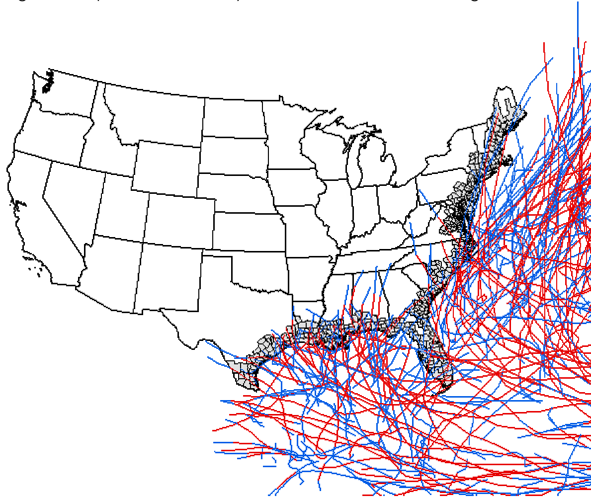
Figure 3: Tropical Storm Activity in the North Atlantic Basin Region since 1970
