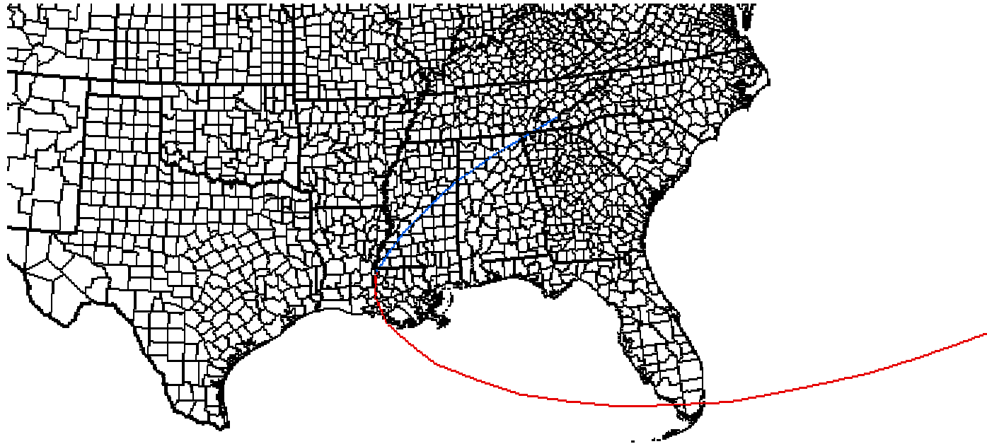
Figure 5: Hurricane Andrew Path
