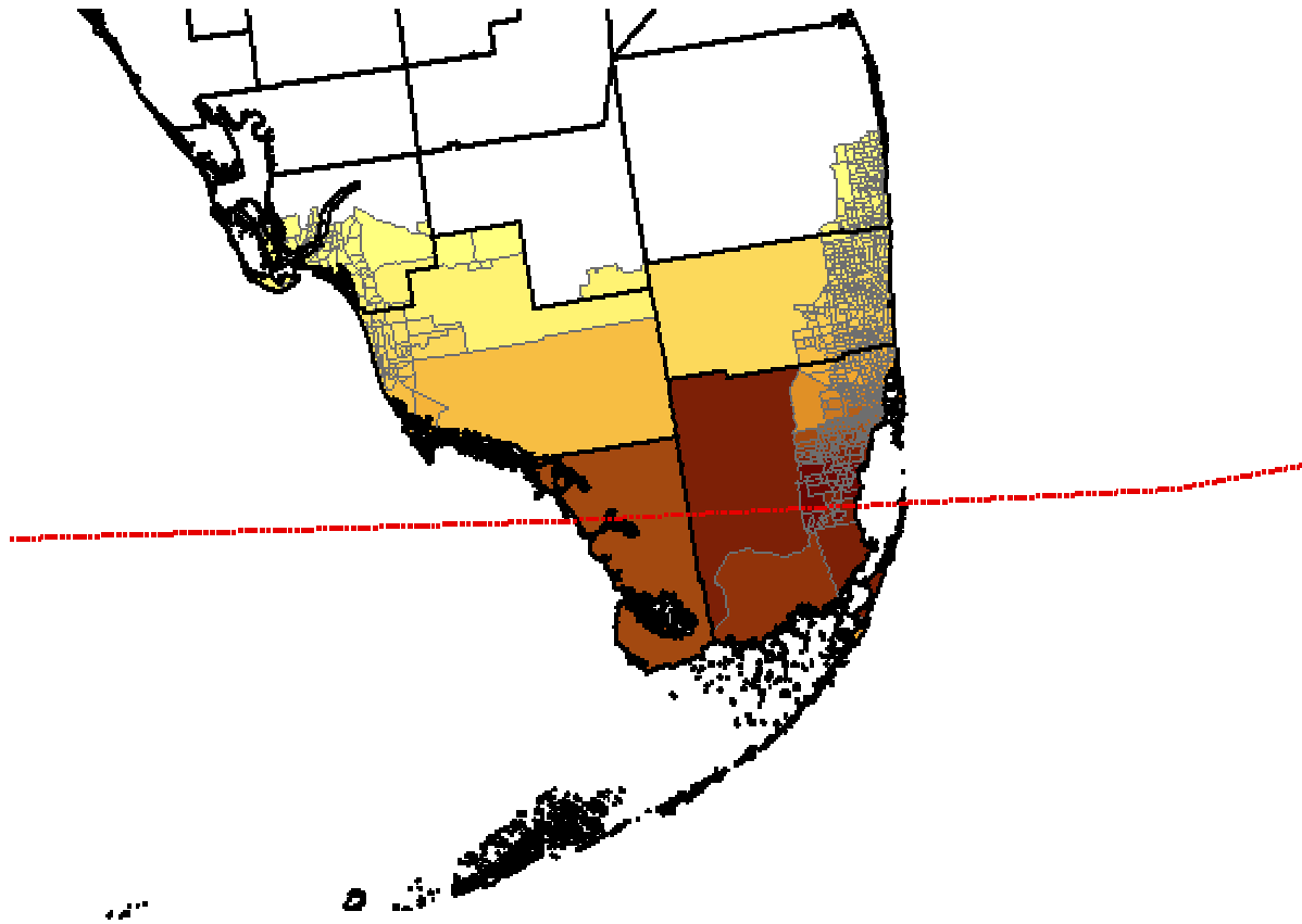
Figure 6: Hurricane Andrew Speed Distribution in Florida
