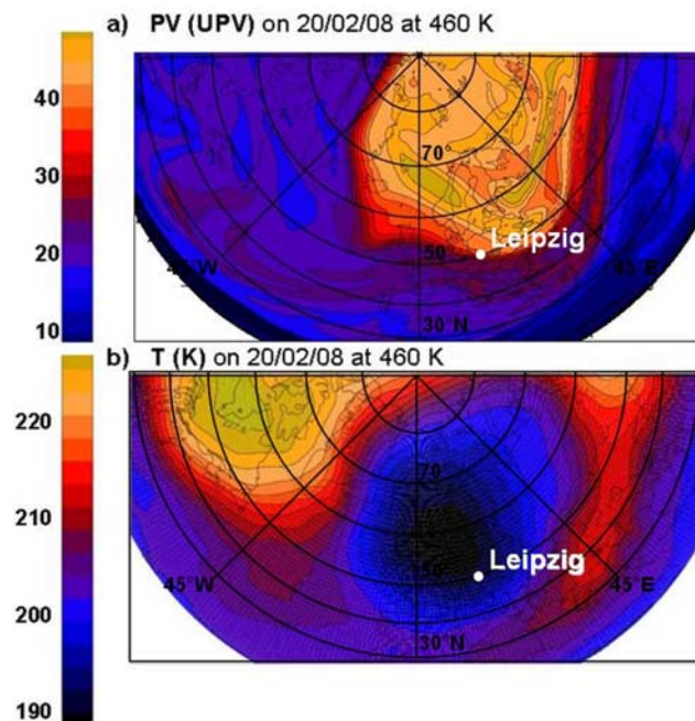
Figure 2. (a) Potential vorticity and (b) temperature on 20 February 2008 at the 460 K level.
