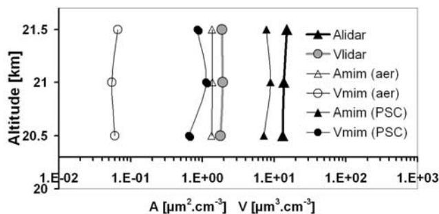
Figure 11. Comparison between the lidar-derived (“lidar”) and model-simulated (“mim”) particle surface area density and volume density. Background aerosol values calculated by MIMOSA- \mu\phi are also plotted (“aer”).
