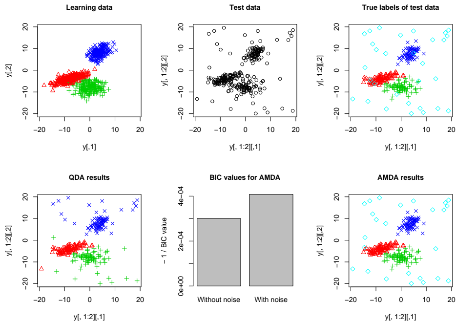
Figure 4: Classification with AMDA of simulated data: 3 observed classes and 1 unobserved noise class (light blue diamonds) in \mathbb{R}^2 .
