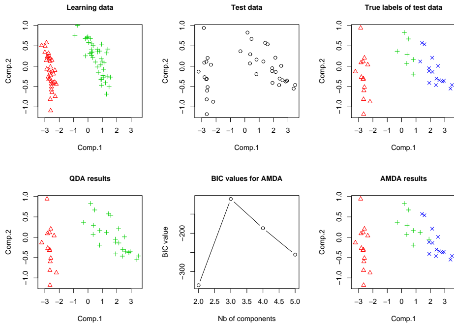
Figure 1: Classification with AMDA of the Iris dataset: the classes “setosa” (red triangles) and “versicolor” (green plus-es) have been observed during the learning phase whereas the class “virginica” (blue crosses) has not.
