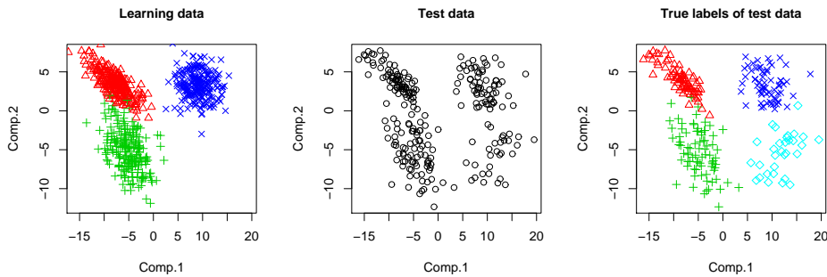
Figure 2: Classification with AMDA of simulated data: 3 observed classes and 1 unobserved class (light blue diamonds) in \mathbb{R}^2 .
