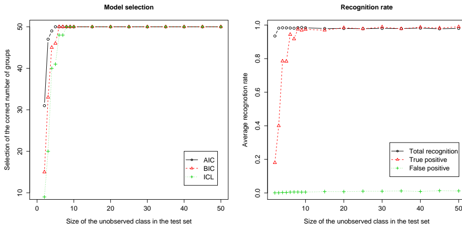
Figure 3: Selection of the number of classes and recognition rates according to the size of the unobserved class with AMDA on simulated data: 3 observed classes and 1 unobserved class in \mathbb{R}^2 .
