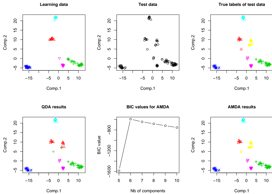
Figure 5: Classification with AMDA of the DNA barcode data: 5 observed bat species and 1 unobserved bat species represented on the two first principal axes.
