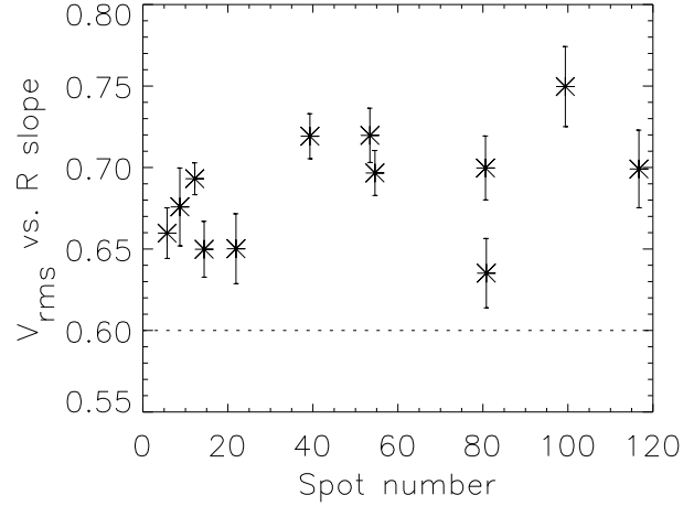
Fig. 4. Slope of \text{Log}(V_{rms}) in cells versus \text{Log}(R) , as a function of the monthly spot number, on the supergranular scale.
