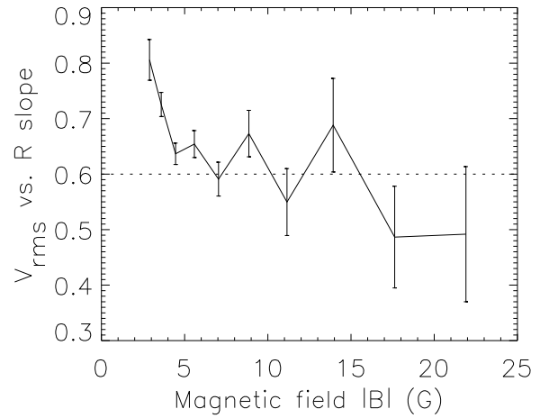
Fig. 5. Slope of \text{Log}(V_{rms}) in cells versus \text{Log}(R) , as a function of the magnetic field level in the cells |B| on the supergranular scale. The horizontal dotted line at 0.6 corresponds to the Bolgiano-Obukhov exponent.
