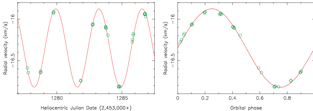
Figure 1. Radial velocities of \tau Boo derived from our ESPaDOs spectra (green circles) as a function of Heliocentric Julian Date (left-hand panel) and orbital phase (right-hand panel, using the ephemeris of equation 1). The radial velocity model plotted here (red full line) corresponds to a circular orbit with an (assumed) velocity semi-amplitude of 467 \text{ m s}^{-1} (Butler et al. 1997) and a (fitted) systemic velocity of -16.348 \text{ km s}^{-1} . Individual error bars on data points ( 15\text{--}20 \text{ m s}^{-1} ) are about as large as the symbol size.
