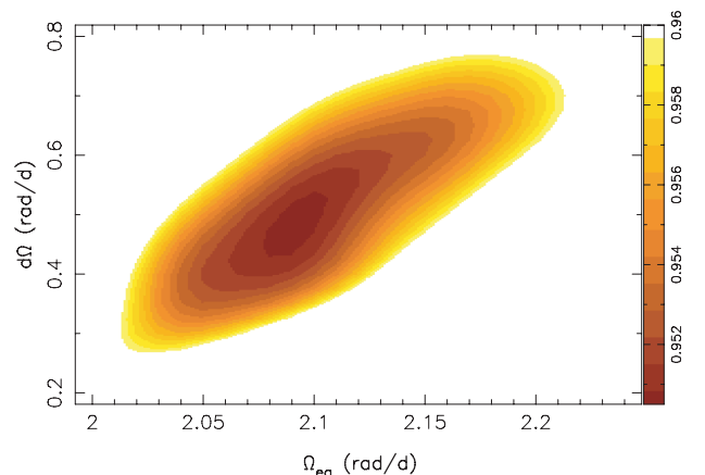
Figure 2. Variation of \chi_r^2 as a function of \Omega_{\text{eq}} and d\Omega , derived from the modelling of our Stokes V data set on \tau Boo. The outer colour contour corresponds to a 1 per cent increase in \chi_r^2 , and traces a 2.7\sigma interval for each parameter taken separately or a 1.7\sigma interval for both parameters as a pair.
