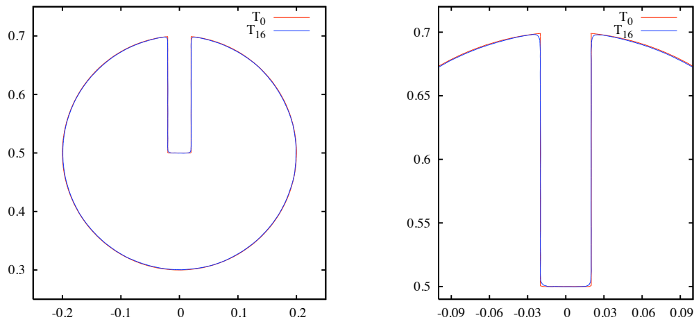
Figure 4. Zalesak slotted disk test: superposition of the slotted disk (blue line) after one complete revolution and the initial one (red line) and zoom on the sharp corners (right).
