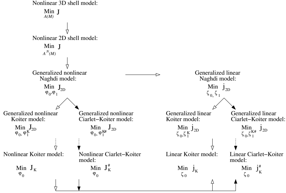
FIGURE 1. Derivation of 2D shell models from the nonlinear 3D shell model. An arrow between two models indicates that the model at the head of the arrow is derived from the model at the neck of the arrow. Dotted arrows indicate that the derivation is not fully justified; see Remarks 6.6 and 7.6. The accuracy of the shell models decreases from top to bottom.
