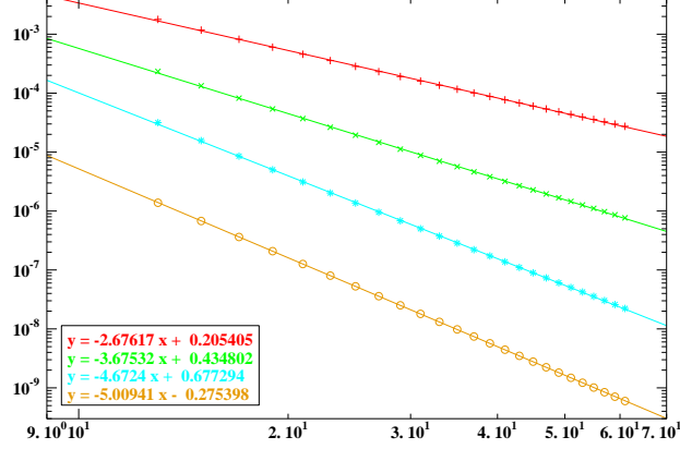
Figure 1: Numerical errors \|u_N - u\|_{H^1} (+), \|u_N - u\|_{L^2} (x), \|u_N - u\|_{H^{-1}} (*), and |\lambda_N - \lambda| (o), as functions of 2N + 1 (the dimension of \tilde{X}_N ) in log scales.
