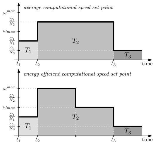
Fig. 4. Different speed set point building: an intuitive vs. an energy efficient computational speed set point behavior
