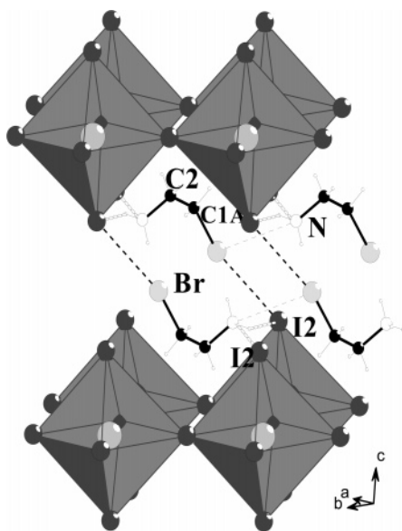
Figure 3. Part of the structure of 2a showing hydrogen and halogen bonding at the organic–inorganic interface.
