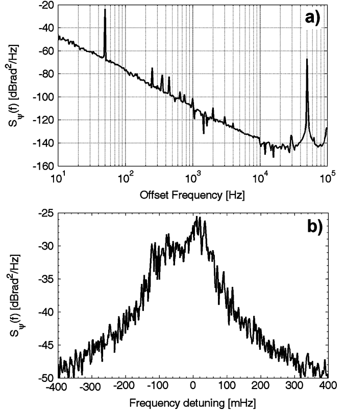
Fig. 6. (a) Experimental phase noise spectrum in a 100 kHz window, showing a noise floor around -145 dBrad 2 /Hz for a microwave power of 10.5 dBm. (b) Enlargement of the spectrum around the first spurious peak at the frequency f_1 = 50594.35 kHz. The maximum of this spurious peak is at -25.5 dBrad 2 /Hz [height of the peak: -119.5 dB], and its -3 dB linewidth is around 40 mHz. All these experimental data are in excellent agreement with the theory. Note that the height of the peak in (a) is not indicative because of insufficient resolution. Also note that the peak at 50 Hz is a parasite peak originating from the electric mains supply.
