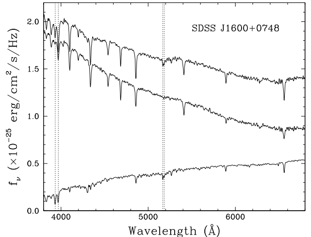
Fig. 1. High-sensitivity ( S/N \sim 300 ) optical spectrum of the J1600+0748 system (upper curve) obtained at the Steward Observatory 2.3-m telescope with the B&C spectrograph. The total exposure time is 44 025 s, gathered over four nights (2007 March 28, May 7, 10, and 11). We used a 400/mm 4889 Å grating in first order and a 2.5" slit, covering the wavelength region 3620–6895 Å at 9 Å resolution. The spectra were wavelength calibrated using 48 non-blended He and Ar lines, and flux calibrated using the standard stars Feige 34 and BD+28 4211, which were observed each night. The middle curve shows the result of our exercise to cleanse the spectrum of the contribution of the late-type main sequence companion (lower curve).
