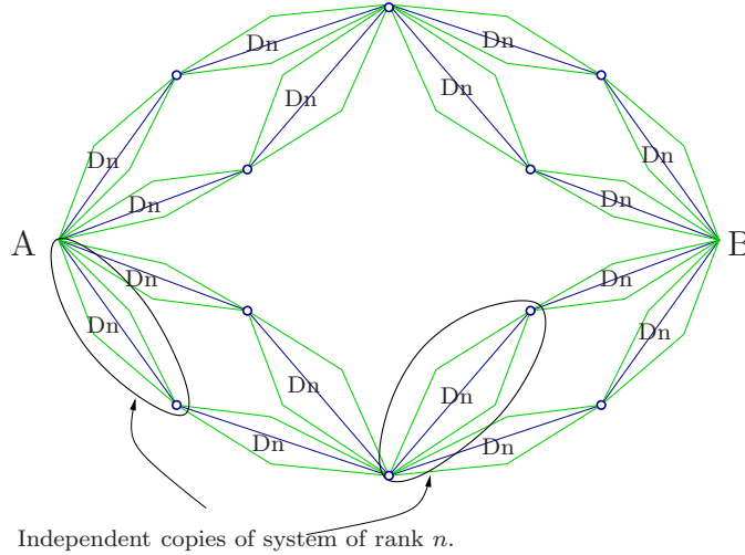
FIGURE 2. On this figure, we scheme how D_{n+m} with its random environment can be seen as independent copies of D_n arrayed as D_m . Here, we have b = s = 2 , each diamond corresponds to a copy of D_n (we can identify it with an edge and get the underlying graph D_2 ). Note that we also have to take into account the environment present on the vertices denoted by circles.
