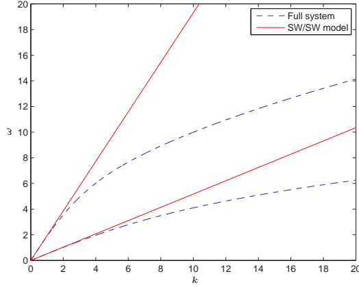
Figure 3: The shallow water/shallow water model dispersion
