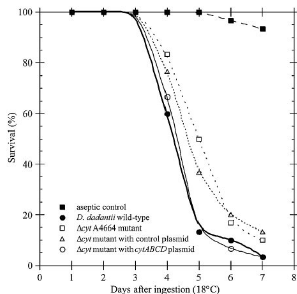
FIG. 4. Survival of pea aphids in response to wild-type, cytABCD -defective, and plasmid-complemented mutants. LT 50 s of strains (in days, at 18°C, standard assay dose): wild type, 4.2 ± 0.25; cyt -defective A4664, 5.0 ± 0.39; A4664 cyt rescued, 4.3 ± 0.21 ( P = 0.011; survival analysis). The A4664 mutant complemented with the control pGEMT plasmid did not differ from its untransformed A4664 control (LT 50 = 4.7 ± 0.24 days).
