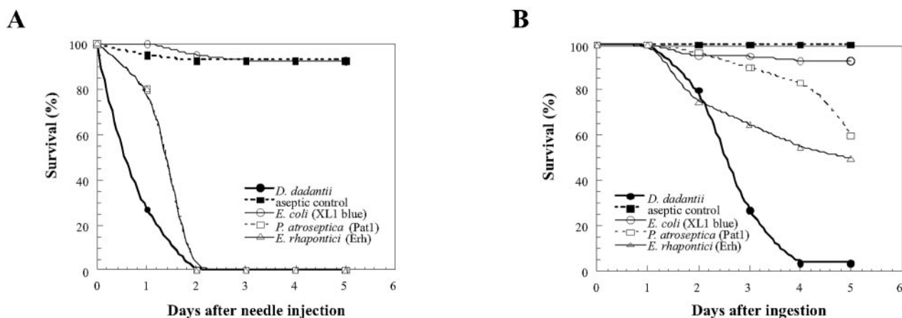
FIG. 1. Aphid survival after infection by Dickeya dadantii ( Erwinia chrysanthemi 3937) and other enteric bacteria. Infection via septic challenge (needle infection) (A) or oral inoculation (ingestion, dose 10^7 bacteria/ml) (B) was evaluated. Bacterial strain abbreviations are as presented in Table 1.
