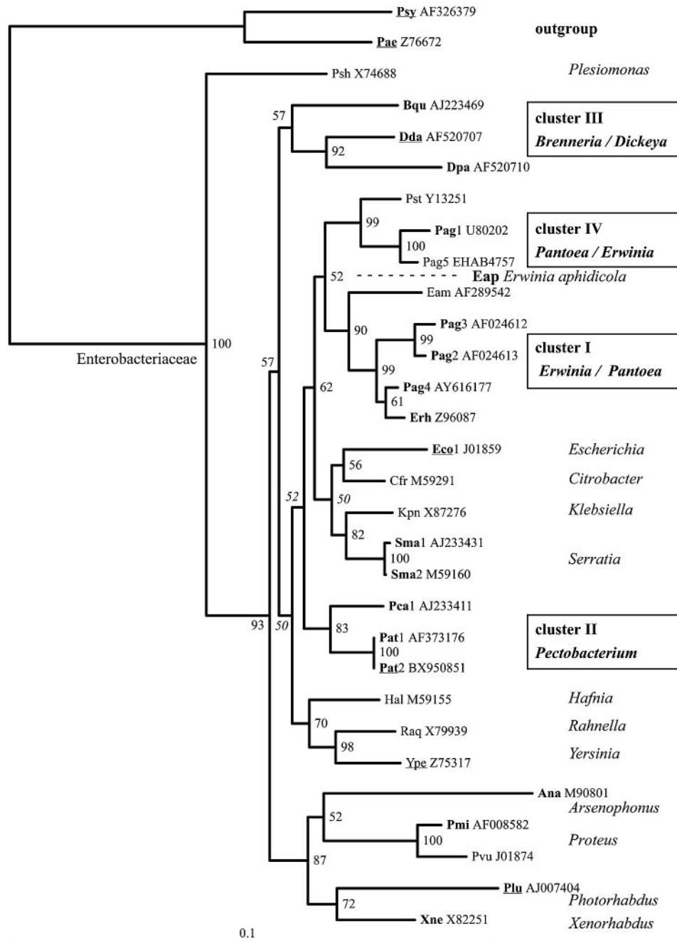
FIG. 2. 16S rRNA phylogenetic tree of tested bacterial strains and additional representative taxa from the Enterobacteriaceae ( Pseudomonas as an outgroup). Taxa with fully sequenced representatives are underlined, and taxa tested in aphid bioassays are in boldface. See the text for the full phylogenetic methodology (1,231 sites, gap removal, neighbor-joining method, Kimura distance, and 1,000 bootstrap replicates). Abbreviations of the additional Enterobacteriaceae strains not included in Table 1: Cfr, Citrobacter freundii ; Eam, Erwinia amylovora ; Hal, Hafnia alvei ; Kpn, Klebsiella pneumoniae ; Pag5, Pantoea agglomerans ; Psh, Plesiomonas shigelloides ; Pvu, Proteus vulgaris ; Raq, Rahnella aquatilis ; Ype, Yersinia pestis . Erwinia aphidicola was positioned manually by a phylogeny on groEL. Clusters I, II, III, and IV refer to the classification of Hauben et al. (33), with a refinement of the positioning of the Dickeya clade.
