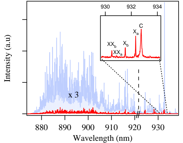
FIG. 1: The full spectrum recorded at 4K showing the inhomogeneous line, with a zoom on the section of interest including two isolated quantum dots ( X_a and X_b ) and their respective bi-excitons ( XX_a and XX_b ), and the cavity mode (C).
