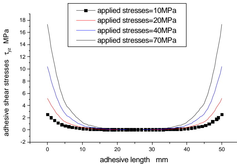
Fig. 5: Variation of the adhesive shear stresses versus the length of the adhesive for different values of the applied stresses. a) Adhesive length=25mm. b) Adhesive length =50mm. (aluminum plates without notch)
