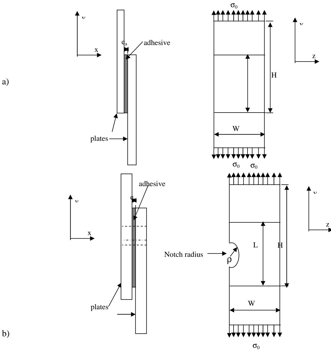
Fig.1: Geometrical model of the bonded structure, a) no notch, b) with notch.
