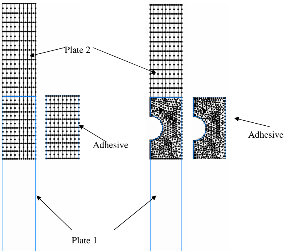
Fig. 2: Typical mesh model of one aluminum plate, a) no notch, b) with notch.
