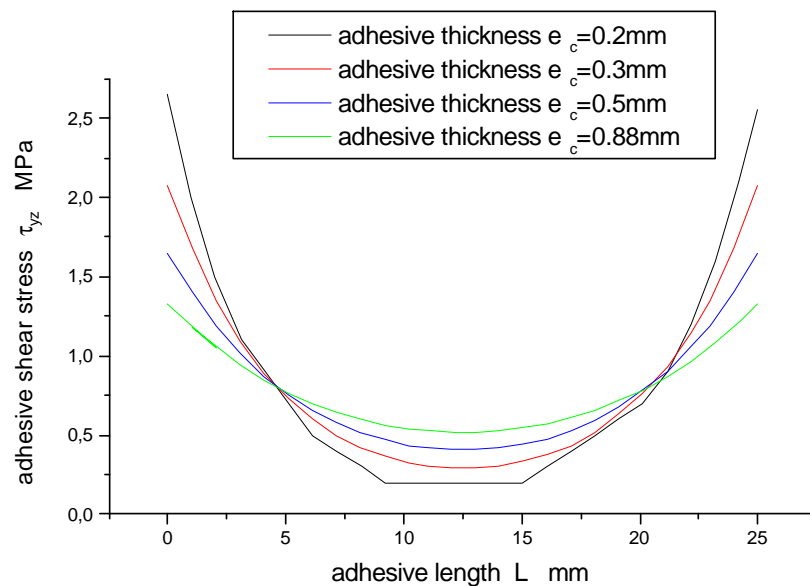
Fig. 3: Distribution of adhesive shear stress according to the length of adhesive for different adhesive thicknesses (without notch and with aluminum plates, applied stress =35 MPa).
