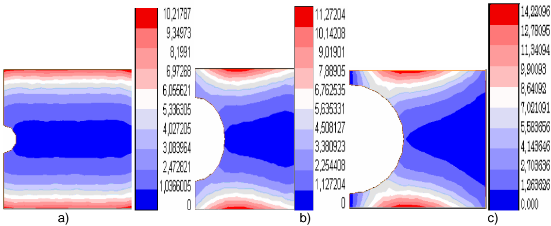
Fig. 7: Contour of the levels of shear adhesive stresses for different notch radius a) \rho=5 mm, b) \rho=15 mm and c) \rho=20 mm ( applied load is 35MPa, adhesive thickness=0.2mm, adhesive length L=25mm width of plate is 25mm)
