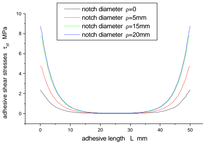
Fig. 9. Distributions of adhesive shear stresses along the adhesive length for different notch diameters; a) adhesive length L=25\text{mm} , b) adhesive length L=50\text{mm} . ( applied stress =35 MPa).
