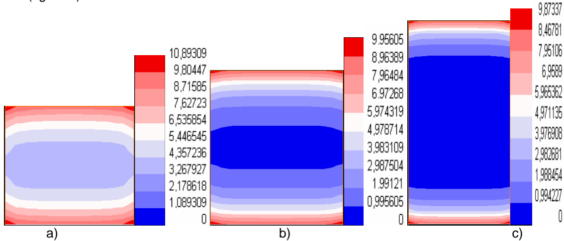
Fig. 6: Contour of the levels of shear adhesive stresses for different adhesive length a) L=12.5mm, b) L=25mm and c) L=50mm (applied load is 35MPa, adhesive thickness=0.2mm, width of plate is 25mm)
