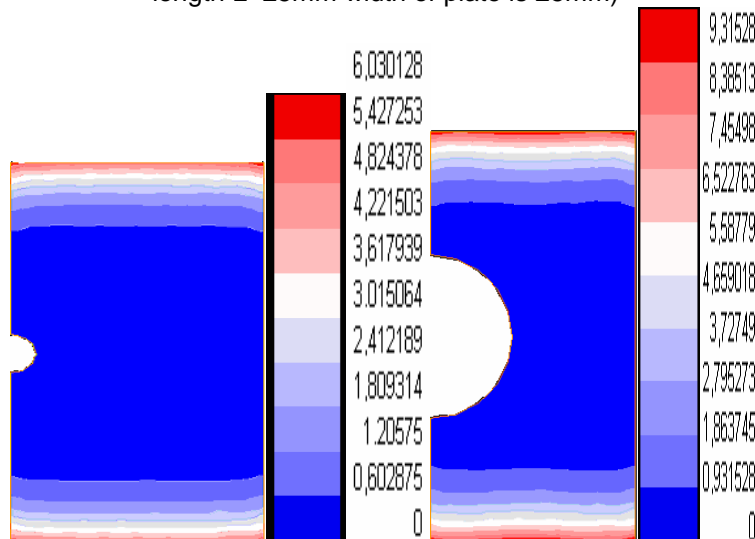
Fig. 7: Contour of the levels of shear adhesive stresses for different notch radius a) \rho=5 mm, b) \rho=15 mm and c) \rho=20 mm ( applied load is 35MPa, adhesive thickness=0.2mm, adhesive length L=25mm width of plate is 25mm)
