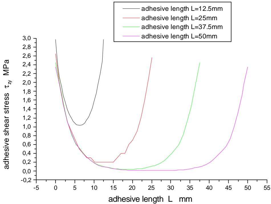
Fig. 4: Adhesive shear stress distribution according to the different adhesive lengths for aluminum plates without notch (adhesive thickness=0.2mm, applied stress =35 MPa).
