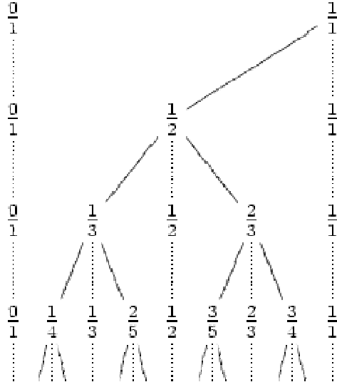
FIGURE 20. The Stern-Brocot tree. Each fraction \gamma on the n -th line is the median of the two fractions closest to \gamma on the n - 1 -st line. The first line consists of 0 and 1 written as 0 = \frac{0}{1} and 1 = \frac{1}{1} . Each rational in [0, 1] is obtained in this way.
