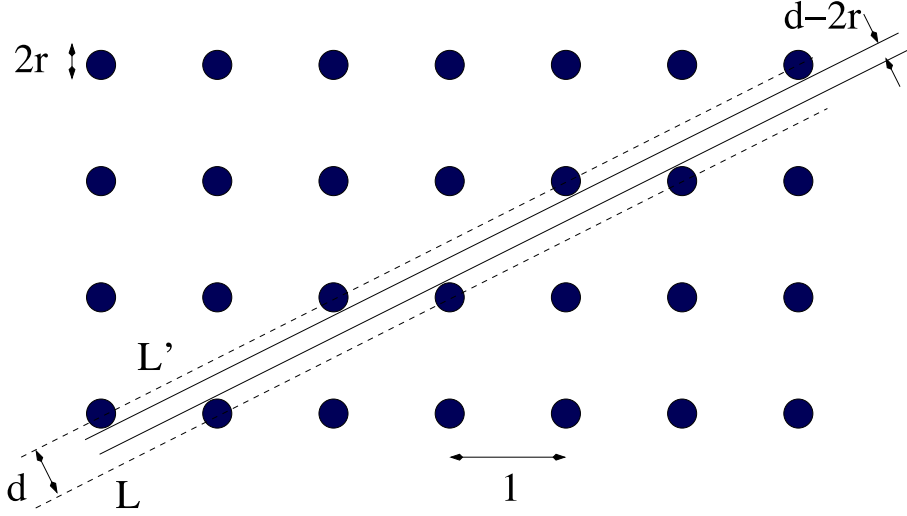
FIGURE 10. A channel of direction \omega = \frac{1}{\sqrt{5}}(2, 1) ; minimal distance d between lines L and L' of direction \omega through lattice points
