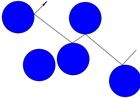
FIGURE 2. The Lorentz gas: a particle path
