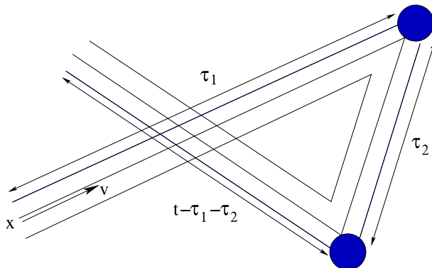
FIGURE 4. The tube T(t, c_1, c_2) corresponding with the third term in the series expansion giving the particle density
