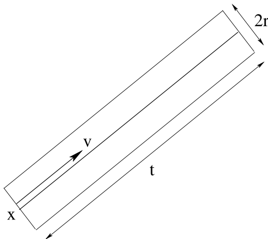
FIGURE 3. The tube corresponding with the first term in the series expansion giving the particle density
