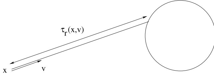
FIGURE 7. The free path length
