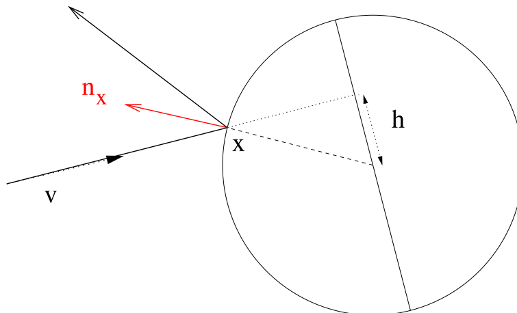
FIGURE 14. The impact parameter h corresponding with the collision point x at the surface of an obstacle, and a direction v
