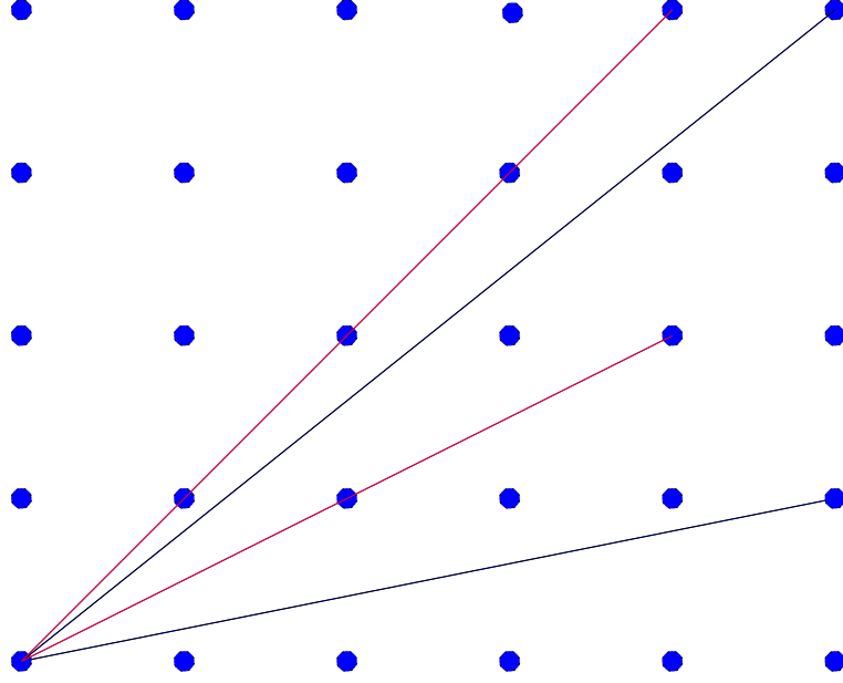
FIGURE 12. Black lines issued from the origin terminate at integer points with coprime coordinates; red lines terminate at integer points whose coordinates are not coprime
