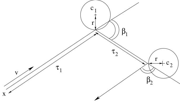
FIGURE 5. The substitution (c_1, c_2) \mapsto (\tau_1, \tau_2, \beta_1, \beta_2)
