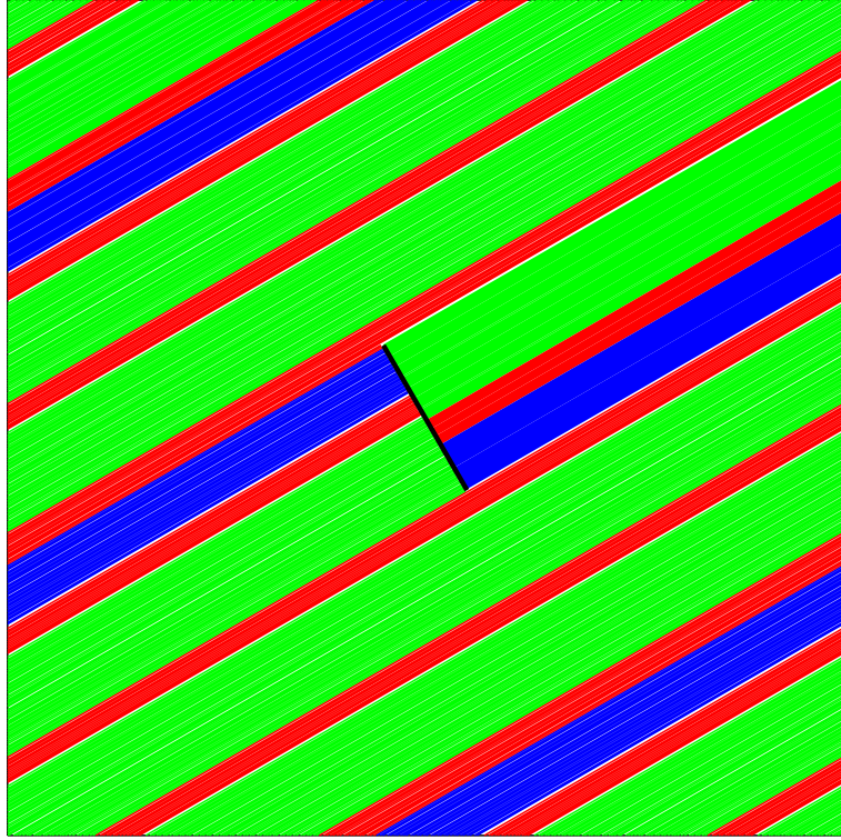
FIGURE 17. The 3-term partition. The shortest orbits are collected in the blue strip, the longest orbits in the red strip, while the orbits of intermediate length are collected in the green strip.
