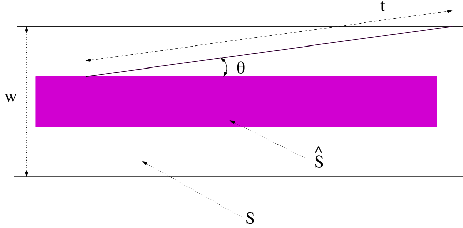
FIGURE 11. Exit time from the middle third \hat{S} of an infinite strip S of width w
