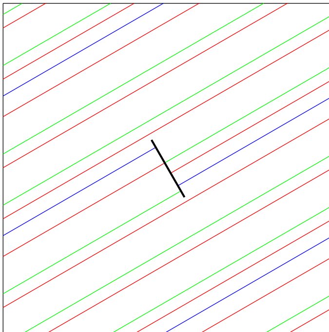
FIGURE 16. Three types of orbits: the blue orbit is the shortest, the red one is the longest, while the green one is of the intermediate length. The black segment removed is orthogonal to the direction of the trajectories.
