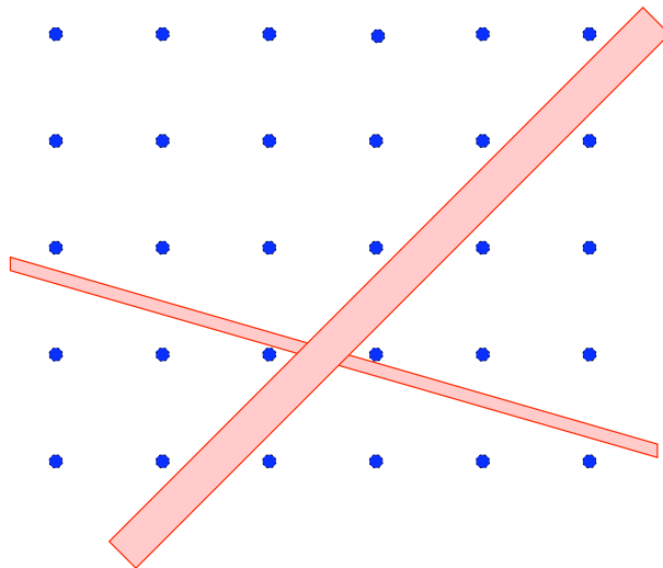
FIGURE 9. Open strips in the periodic billiard table that never meet any obstacle
