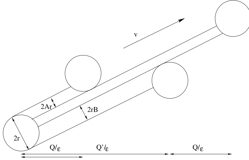
FIGURE 19. Collision pattern seen from the surface of one obstacle. Here, \varepsilon = 2r/v_1 .
