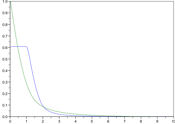
FIGURE 13. Graph of \Phi(t) (blue curve) and g(t) = \Phi''(t) (green curve)
