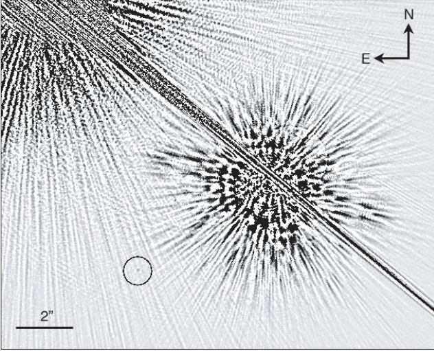
Fig. 3. Extract of an HST-ACS coronagraphic image of \alpha Cen B showing the bright background star #167 (circled) that was used to transfer the reference astrometric coordinates of \alpha Cen B to the NACO images. The saturated source in the upper left corner is \alpha Cen A.
