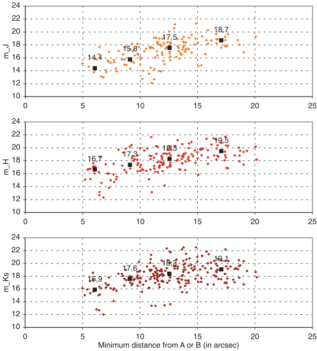
Fig. 6. Apparent magnitudes of the detected objects, as a function of their minimum angular separation with \alpha Cen A or B. The solid squares correspond to the median magnitude of the objects detected in the 5–7'', 7–10'', 10–15'', and 15–20'' domains, respectively. The corresponding magnitude is indicated in each case.
