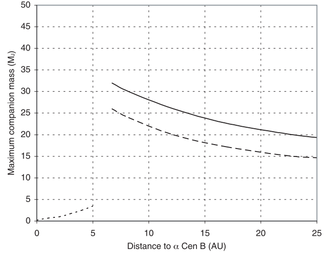
Fig. 7. Maximum mass of possible companions to \alpha Cen B within the area explored by NACO imaging (encircled zone in Fig. 2, bottom ). The solid curve corresponds to the median magnitude of the detected sources (Fig. 6, bottom ) and the dashed line to the faintest detected objects. The dotted curve corresponds to the mass limit obtained by Endl et al. (2001) from radial velocity measurements.
