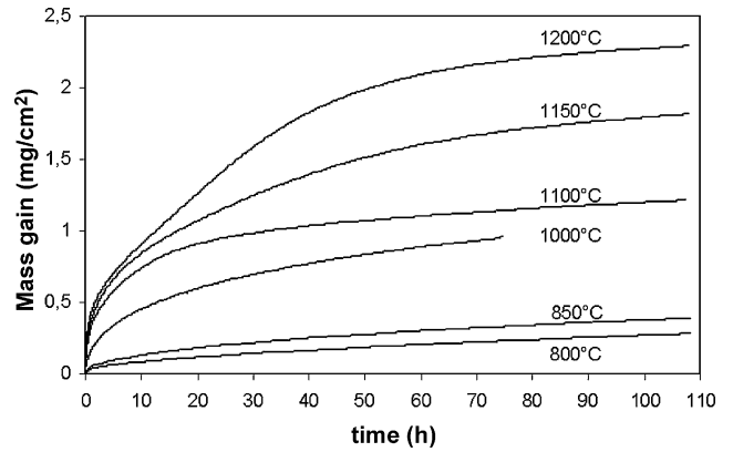
Fig. 5. Isothermal TGA curves showing the oxidation kinetic of the \text{Si}_3\text{N}_4 -TiN ceramic in air between 800 and 1200 °C.
