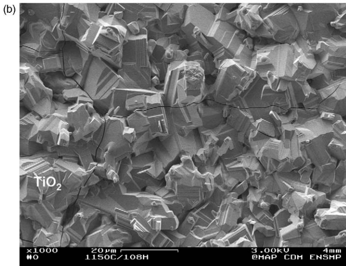
Fig. 3. Micrographs of the \text{Si}_3\text{N}_4 -TiN surface after a 108 h oxidation treatment at 800 °C (a) and 1150 °C (b).
