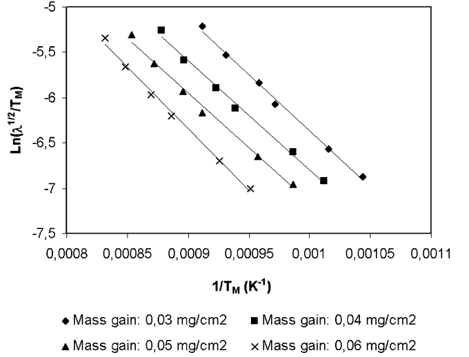
Fig. 9. \ln(\lambda^{1/2}/T_M) = f(1/T_M) curves at constant mass gain deduced from non-isothermal TGA results.
