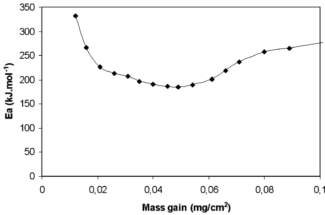
Fig. 10. Activation energy calculated from Fig. 9 for oxygen diffusion through \text{TiO}_2 phase.
