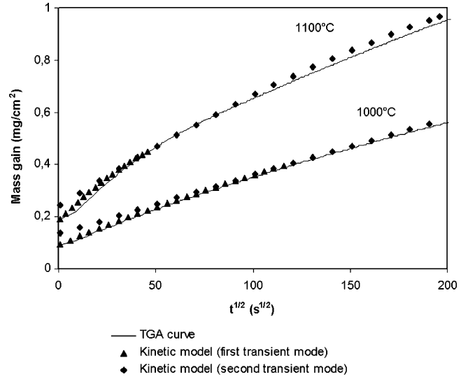
Fig. 14. Comparison between the kinetic model and the TGA curves at the beginning of the isothermal oxidation (transient modes).
