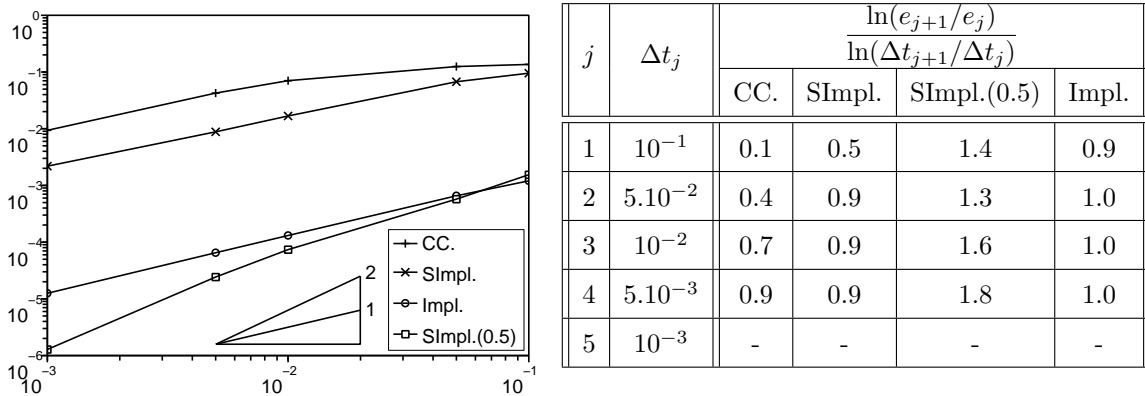
FIGURE 6. Errors e_j(t) = |\mathbf{c}^{\Delta t_j}(t, \cdot) - \mathbf{c}^{\Delta t_{\text{ref}}}(t, \cdot)|_{(L^2(\Omega))^3} at time t = 3.8 as a function of the time step \Delta t_j (left) and convergence rates (right) obtained for the different schemes
