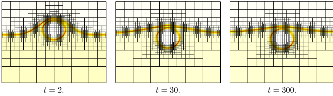
FIGURE 16. Evolution of the interface position for \Delta t = 10^{-3} using the SImpl. scheme.
