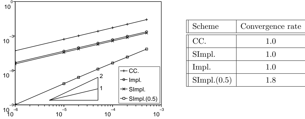
FIGURE 2. Errors e_j(t) = |\mathbf{c}^{\Delta t_j}(t, \cdot) - \mathbf{c}^{\Delta t_{\text{ref}}}(t, \cdot)|_{(L^2(\Omega))^3} at time t = 0.01 as a function of the time step \Delta t_j (left) and convergence rates (right) obtained for the different schemes
