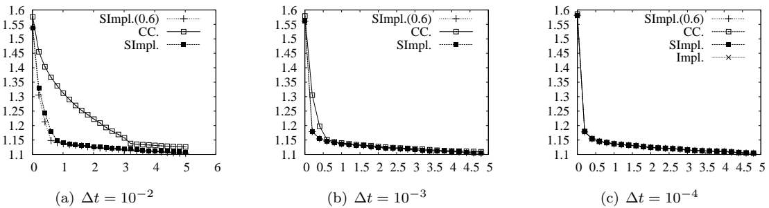
FIGURE 19. Time evolution of energy in a partial spreading situation
