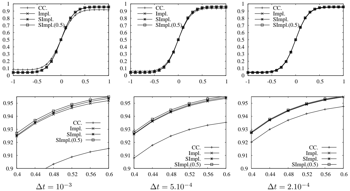
FIGURE 3. First order parameter c_1 as a function of the space variable x at time t = 0.01 . Top: x \in [-1, 1] , Bottom: x \in [0.4, 0.6] (zoom)
