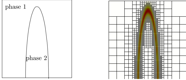
FIGURE 7. Configuration of test case (left) and initial position of interface (right)
