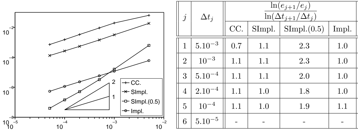
FIGURE 9. Errors e_j(t) = |\mathbf{c}^{\Delta t_j}(t, \cdot) - \mathbf{c}^{\Delta t_{\text{ref}}}(t, \cdot)|_{(L^2(\Omega))_3} at time t = 1.5 as a function of the time step \Delta t_j (left) and convergence rates (right) obtained for the different schemes
