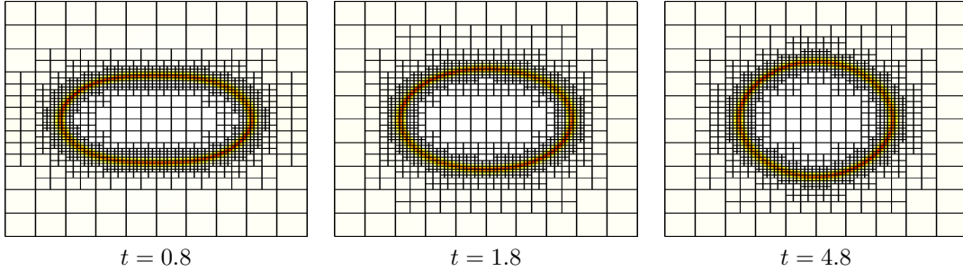
FIGURE 5. Evolution of the interface position using the Impl. scheme with \Delta t = 5.10^{-4}
