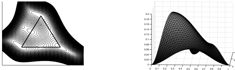
FIGURE 17. Cahn-Hilliard potential F using barycentric coordinates
