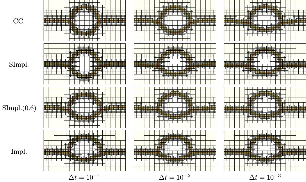
FIGURE 14. Influence of schemes on bubble shape at t = 2 .
