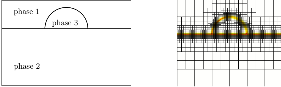
FIGURE 15. Configuration of test case (left) and initial position of interface (right)
