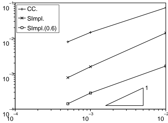
FIGURE 18. Errors e_j(t) = |\mathbf{c}^{\Delta t_j}(t, \cdot) - \mathbf{c}^{\Delta t_{ref}}(t, \cdot)|_{(L^2(\Omega))^3} at time t = 3.8 as a function of the time step \Delta t_j (left) and convergence rates (right) obtained for the different schemes
