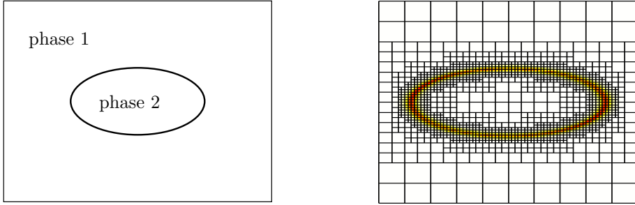
FIGURE 4. Configuration of test case (left) and initial position of interface (right)
