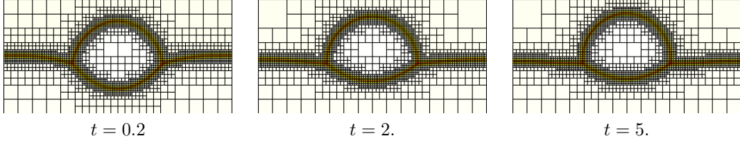
FIGURE 11. Evolution of the interface position for \Delta t = 10^{-4} using the Impl. scheme.
