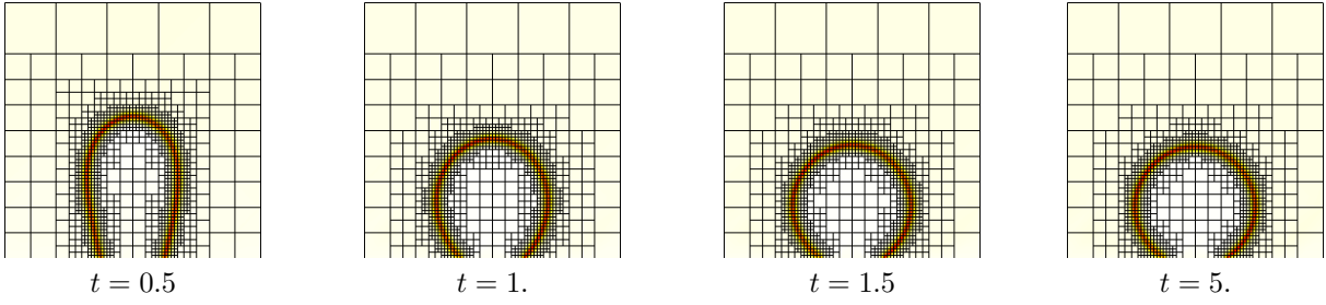
FIGURE 8. Evolution of the interface position using the Impl. scheme with \Delta t = 5.10^{-5}
