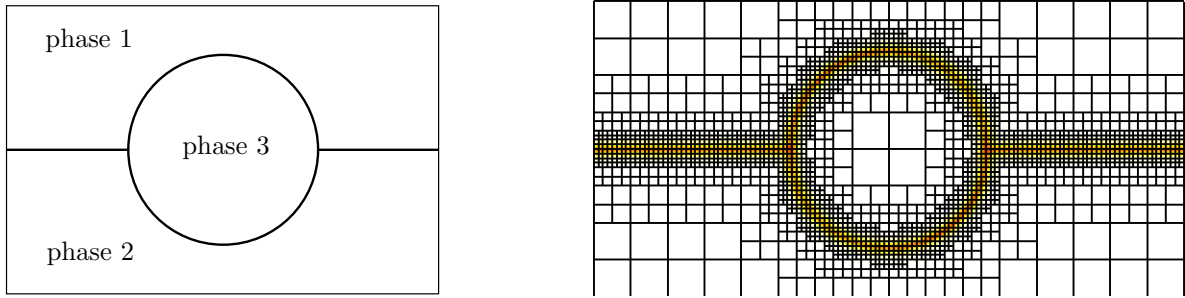
FIGURE 10. Configuration of test case (left) and initial position of interface (right)
