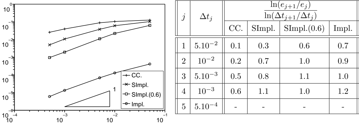
FIGURE 12. Errors e_j(t) = |\mathbf{c}^{\Delta t_j}(t, \cdot) - \mathbf{c}^{\Delta t_{\text{ref}}}(t, \cdot)|_{(L^2(\Omega))^3} at time t = 2 , as a function of the time step \Delta t_j (left) and convergence rates (right) obtained for the different schemes
