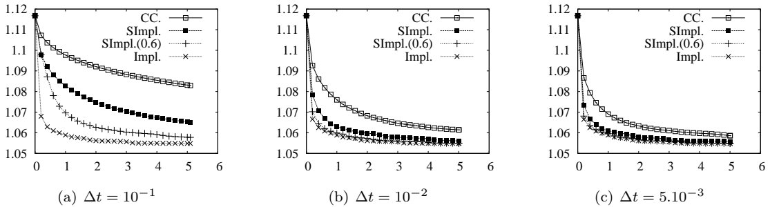
FIGURE 13. Time evolution of energy in a partial spreading situation
