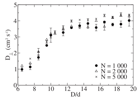
FIG. 13. Evolution of D_{\perp} versus D/d for different values of N . The results are obtained with H/D=14 , D=20 mm, e_1=0.84 , and e_2=0.99 . To improve the readability, only significant error bars are displayed.
