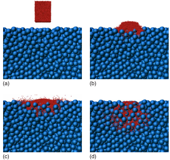
FIG. 9. (Color online) Snapshots of flow of 20 000 particles through a porous medium. Note that for convenience only half system is represented.
