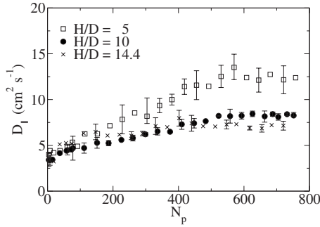
FIG. 8. Dispersion coefficients in the flow direction determined with Eq. (11), versus the parameter N_p for three different packing heights H . In these experiments, we use small steel beads of diameter d=1 mm inside a packing of glass beads of diameter D=16 mm (size ratio D/d=16 ). In order to improve visual quality of the figure, all error bars are not displayed.
