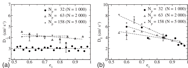
FIG. 15. Evolution of (a) D_{\perp} and (b) D_{\parallel} with e_1 for N=1000 , N=2000 , and N=5000 . The results are obtained with H/D=14 , D/d=10 , D=20 mm, and e_2=0.99 . Unweighted linear least-squares regressions are also represented.
