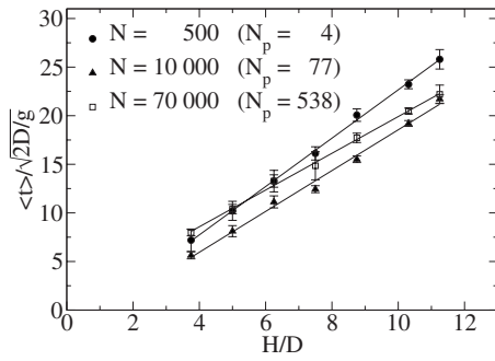
FIG. 5. Mean transit time dependency on H/D for N=500 , N=10\,000 , and N=70\,000 . Results obtained with steel percolating particles of d=1 mm inside glass beads of diameter D=16 mm. Linear fits are also represented.
