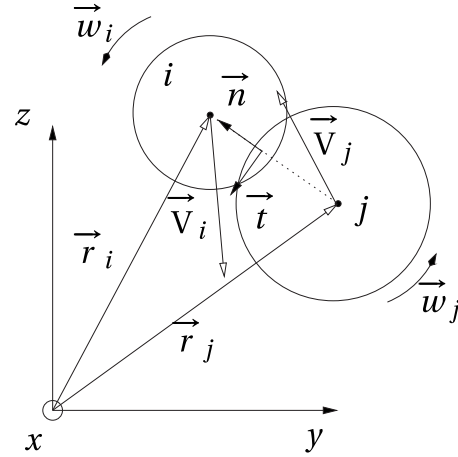
FIG. 2. Illustration of contact between two soft overlapping spheres i and j in the MD approach. Notations used in this paper are also mentioned.
