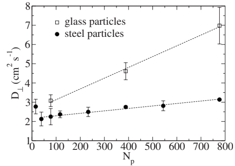
FIG. 7. Evolution of transverse dispersion coefficient D_{\perp} versus N_p . The experiments were performed with small steel (●) and glass (□) beads of diameter d=1 mm through a porous medium made with glass bead of diameter D=16 mm (size ratio D/d=16 ). We have also represented unweighted linear least-squares regressions.
