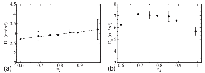
FIG. 16. Evolution of (a) D_{\perp} and (b) D_{\parallel} versus e_2 for N=2000 , D/d=10 , D=20 mm, H/D=14 , and e_1=0.84 . An unweighted linear least-squares regression is represented in case (a).
