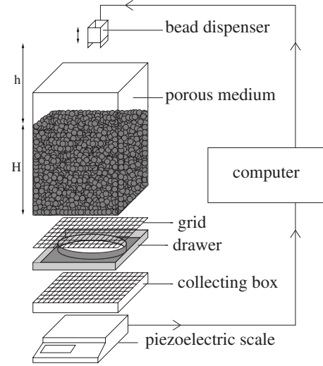
FIG. 1. Schematic description of the experimental setup. The small bead dispenser is placed at h from the top of the porous media of an height H . The collecting box is put on the scale.
