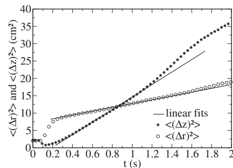
FIG. 10. Time evolutions of \langle(\Delta z)^2\rangle and \langle(\Delta r)^2\rangle versus time obtained by the MD model of soft spheres, with N=8000 , D/d=10 , D=20 mm, e_1=0.84 , e_2=0.99 , and H/D=14 . Linear fits obtained with unweighted least-squares method are represented. The linear evolution of \langle(\Delta z)^2\rangle is observed between 0.2 and 1 s as shown by the straight line. After 1 s the decrease in the moving particles amount explains the divergence which is only an artifact of the calculus method. The same behavior is observed on evolution of \langle(\Delta r)^2\rangle but divergence starts to be visible after 1.5 s.
