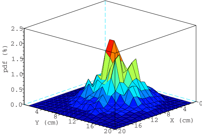
FIG. 3. (Color online) Distribution function of particle positions at the exit of the porous medium for a launch of 10 000 glass particles of mass m_s = 2.1 \times 10^{-3} g and with a porous medium of height H/D = 8.125 .
