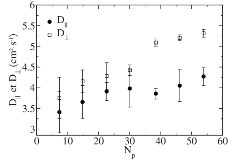
FIG. 12. Evolution of dispersion coefficients versus N_p for a size ratio D/d=16 . Error bars are shown for accuracy analysis. Results are obtained with H/D=14 , D=20 mm, e_1=0.84 , and e_2=0.99 .
