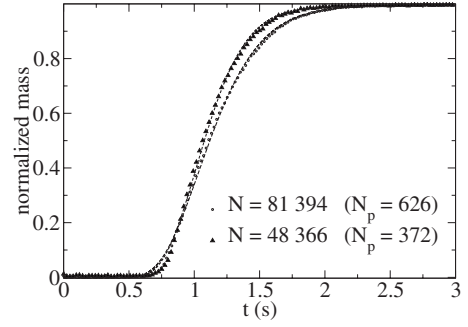
FIG. 4. Normalized mass measurements delivered by the piezoelectric scale. A fit with Eq. (11), and determined with unweighted least-squares method, is also represented with continuous lines. N corresponds to the number of falling steel particles and N_p is the rescaled value, which was defined in Sec. II. Here H/D = 10 .
