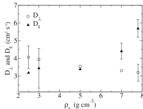
FIG. 17. Evolution of D_{\parallel} and D_{\perp} versus density \rho_s of the small particles for N=2000 , D/d=10 , D=20 mm, H/D=14 , e_2=0.99 , and e_1=0.84 .
