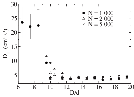
FIG. 14. Evolution of D_{\parallel} versus D/d for different values of N . Results have been obtained by the MD model of soft spheres with H/D=14 , D=20 mm, e_1=0.84 , and e_2=0.99 .
