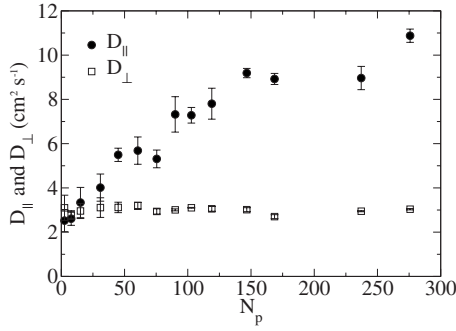
FIG. 11. Evolution of dispersion coefficients versus N_p for a size ratio D/d=10 . These results have been obtained with H/D=14 , D=20 mm, e_1=0.84 , and e_2=0.99 . Error bars are also represented.
