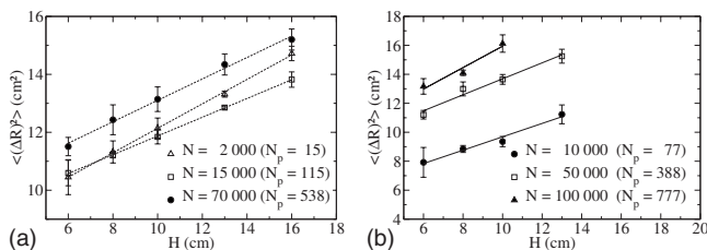
FIG. 6. Variance of the particle distribution function in the transverse direction at the output of the porous medium versus H for different numbers of falling particles. In these experiments, we used small steel beads (a) and glass ones (b) of diameter d=1 mm inside packings of glass beads of diameter D=16 mm (i.e., size ratio D/d=16 ). Unweighted linear least-squares regressions are also represented.
