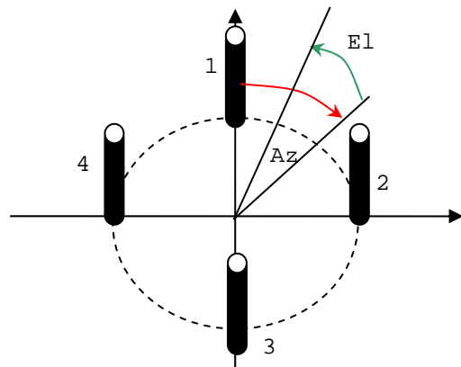
Figure 7: Array configuration.
