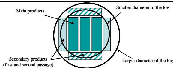
Fig. 3. The cutting plan
