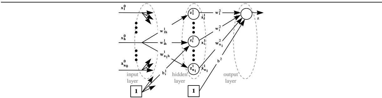
Fig. 2. Architecture of the multilayer perceptron
