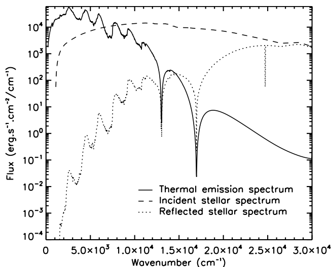
Fig. 3. Reflected and thermal emission spectra of the static disk-averaged solution for the nominal boundary condition, on a logarithmic scale. The incident stellar spectrum is shown for comparison.
