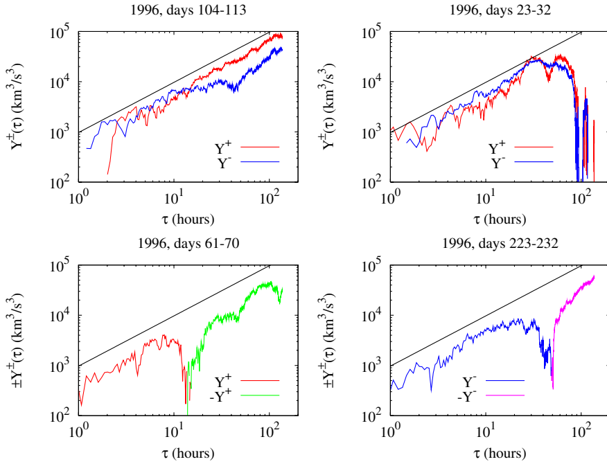
FIG. 1 (color online). The scaling behavior of Y^{\pm}(\tau) as a function of the time scale \tau for four different periods we examined. Different colors of the curves refer to positive and negative values of the mixed structure functions Y^{\pm}(\tau) and thus of \epsilon^{\pm} . The full black lines correspond to linear scaling laws to guide the eye.
