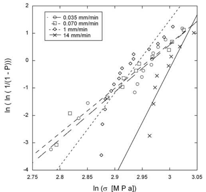
Figure 2. Same as Figure 1 but with the cumulative probability of failure transformed in its linear form provided by equation (7).
