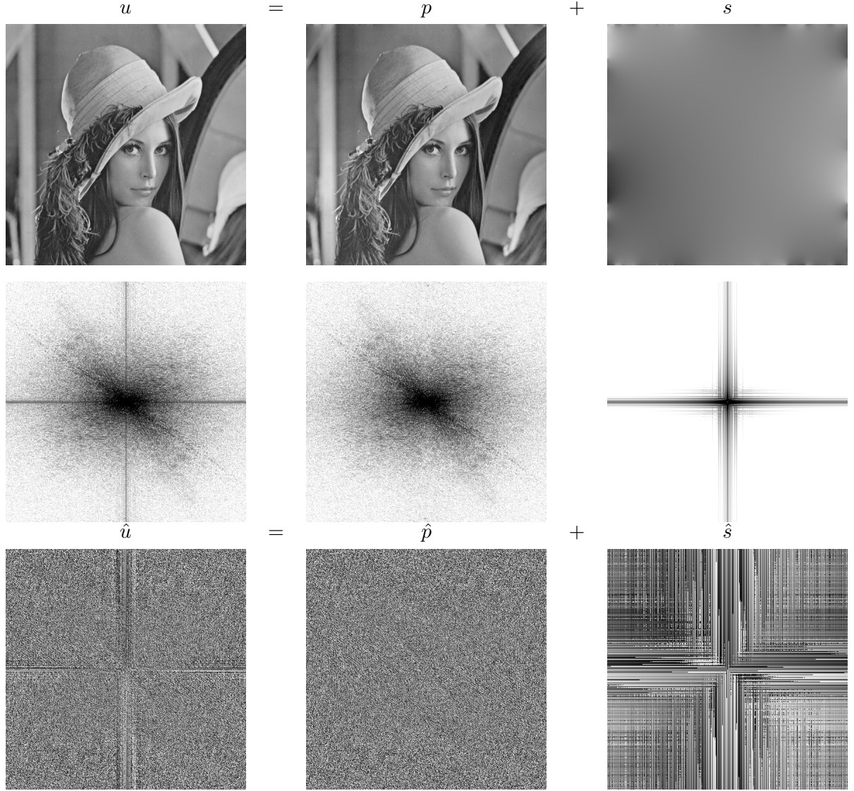
Figure 3: The original Lena image u (top row, left column) is decomposed into its periodic component p (top row, middle column) and its smooth component s (top row, right column). The Fourier spectrum of each of these three images is represented underneath: the modulus in log scale appears on the middle row, and the argument (phase) on the bottom row. As we can see, the periodic component captures not only most of the visual information (the difference between u and p being noticeable only at large scales), but also the relevant data for DFT purposes, allowing a pleasant artifact-free restoration of the spectrum of u . On the contrary, the smooth component mainly gather the frame border discontinuities in the image domain, and equivalently the consequent “cross structure” in the Fourier domain. Note that the mean value of the smooth image has been shifted to 128 for display purposes.
