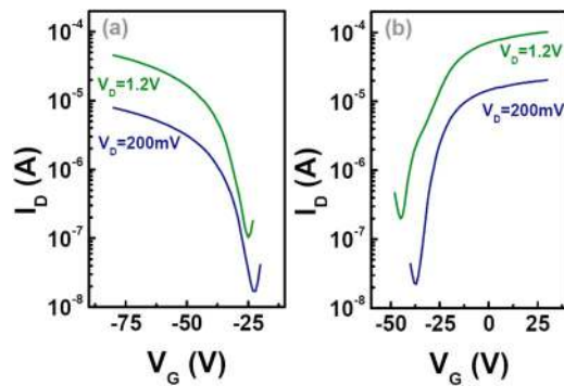
FIG. 4. (Color online) Pseudo-MOSFET drain-current ( I_D - V_G ) measurements in (a) accumulation and (b) inversion regimes for V_D=200 mV and V_D=1.2 V.
