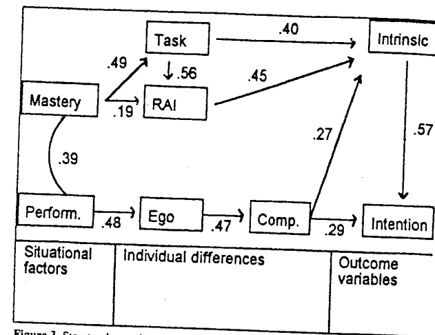
Figure 3. Structural equation model for Model 1a for the football/netball data. Curved lines represent relationships with no specified causal influence. All path coefficients significant at p < .01 .
