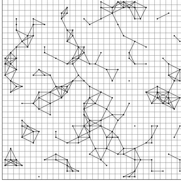
Figure 1: Two-dimensional geometric graph with radius r = \frac{\sqrt{5}}{32} , and vertex probability p = 0.2 .
