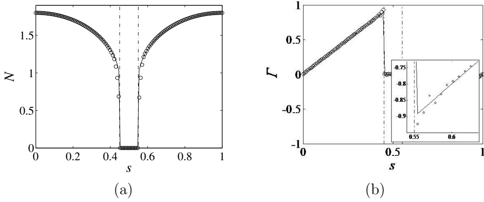
Figure 6: One dimensional spectral solution profiles (circles) and analytical solution (solid line) for density N (a) and parallel momentum \Gamma (b), with the magnification of the momentum profile closed to the limiter. Vertical dotted lines indicate the limiter location. Fourier mode n = 128 , penalization parameter \eta = 10^{-7} and filtering coefficient \alpha = 10 are used.
