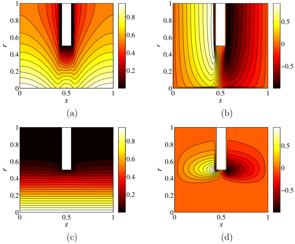
Figure 11: Contours plot of density (a,c) and particle flux (b,d) in steady state conditions given by Sc = 1 and A = 50 . The radial extension of the edge region is between r = 0 and r = 0.5 and the SOL is defined between r = 0.5 and r = 1 . Strong diffusive transport at Pe = 100 (a,b) and weak diffusive transport at Pe = 5000 (c,d). Fourier modes n = 128 and n_r = 50 , penalization parameter \eta = 10^{-7} and filtering coefficient \alpha = 10 are used.
