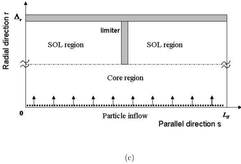
Figure 1: Geometry of the model. (a) Schematic representation of a toroidal tokamak with a circular poloidal section with a toroidal limiter. The white line shows an open magnetic field line of length L_{\parallel} . (b) Poloidal cut of the vacuum chamber. The inner white annulus shows the core region not taken into account. (c) Two-dimensional computational domain including the transition between the core and the SOL region up to the wall.
