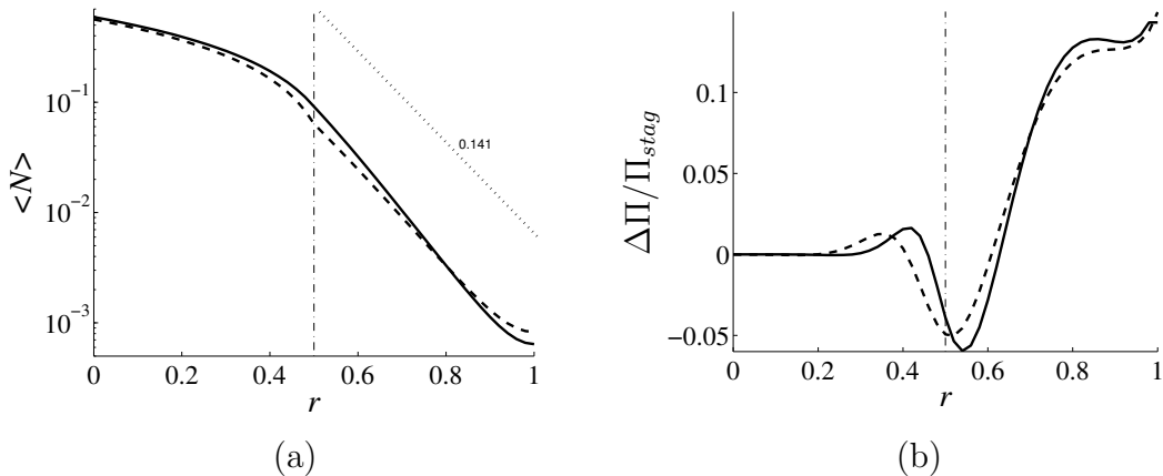
Figure 12: Mean density (a) and total pressure variation from the stagnation point close to the limiter (b) profiles in the radial direction for Sc = 1, Pe = 5000, A = 50 . Solutions from reference [33] with a limiter with zero thickness imposed by surface Bohm boundary conditions (solid line), the present penalization (dashed line) and the analytical slope [33] (dotted line). The interaction between the core and the SOL is for r = 0.5 . Fourier modes n = 128 and n_r = 50 , penalization parameter \eta = 10^{-7} and filtering coefficient \alpha = 10 are used.
