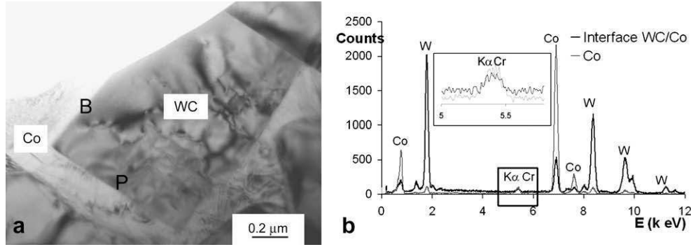
Fig. 10. (a) TEM image of the analysed area in WC-13Co, Cr, C sintered at 1200 °C. The observation direction of the WC grain is close to \langle 11 - 20 \rangle (b) Example of EDS spectra of the Co binder and of the prismatic WC/Co interface called P .
