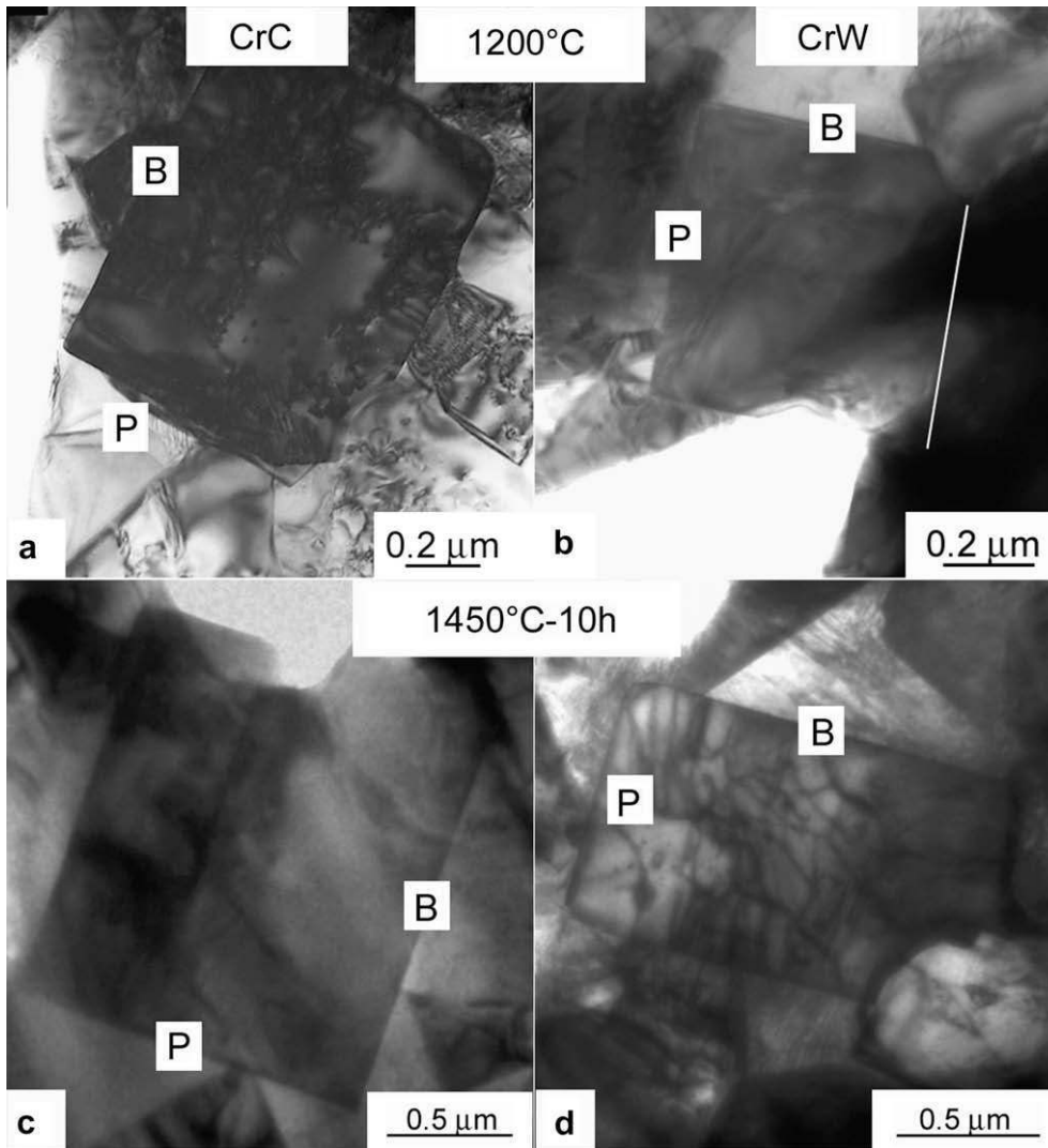
Fig. 6. TEM images of the WC grains viewed along the [11\bar{2}0] direction in the alloys sintered at 1200 °C (a) WC-13Co, Cr, C with k = 0.80 and (b) WC-13Co, Cr, W with k = 1.08 , and in the alloys sintered for 10 h at 1450 °C (c) WC-34Co, C, Cr (10 h) with k = 0.81 (d) WC-34Co, W, Cr with k = 0.61 . The letters B and P indicate the basal and prismatic facets of the WC grains.
