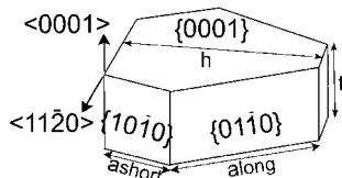
Fig. 1. Morphology of WC grains in WC-Co alloys showing the (0001) basal and {10-10} prismatic facets.
