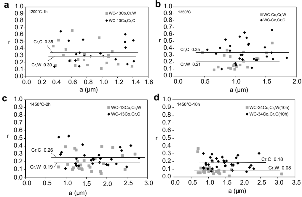
Fig. 5. r values versus the grain size recorded after heating at (a) 1200 °C, (b) 1350 °C and (c) 1450 °C for 2 h in WC–13Co, Cr, C and WC–13Co, Cr, W and (d) after 10 h at 1450 °C in WC–34Co, Cr, C and WC–34Co, Cr, W.
