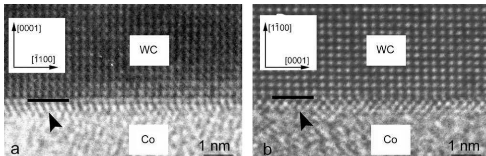
Fig. 11. HRTEM images of WC/Co interfaces viewed along the \langle 11 - 20 \rangle direction of WC in WC-13Co, Cr, C sintered for 1 h at 1200 °C. The arrows indicate a thin crystalline layer about 1 nm in thickness at the interface between WC and Co (a) at the basal and (b) at the prismatic facets of the WC grains.
