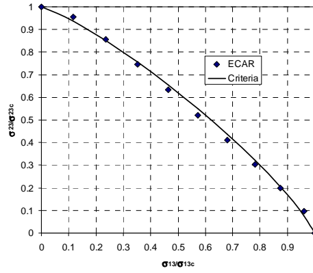
Fig. 5 : Enveloppe de rupture \sigma_{23} - \sigma_{13} , Nomex ECA, ECA-R 48 Kg m-3 \sigma_{23} - \sigma_{13} Stress failure predictions for ECA and ECA-R 48 Kg m-3
