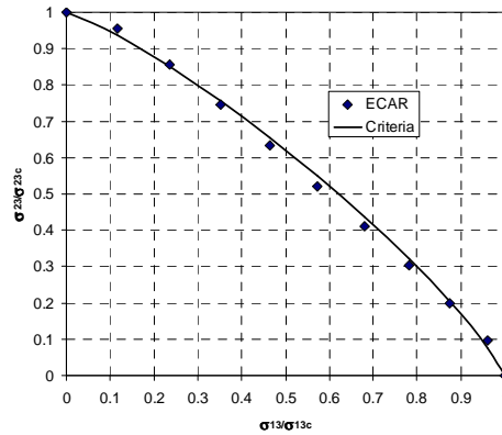
Fig. 6 :: Enveloppe de rupture \sigma_{23} - \sigma_{13} , Nomex ECA, ECA-R 48 Kg m-3 \sigma_{23} - \sigma_{13} Stress failure predictions for ECA and ECA-R 48 Kg m-3
