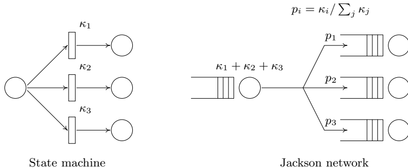
Fig. 6. From (generalized) state machine to Jackson network.
