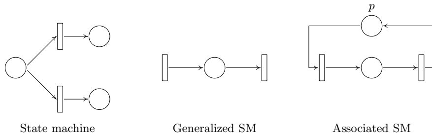
Fig. 5. State machine, generalized state machine and associated state machine.
