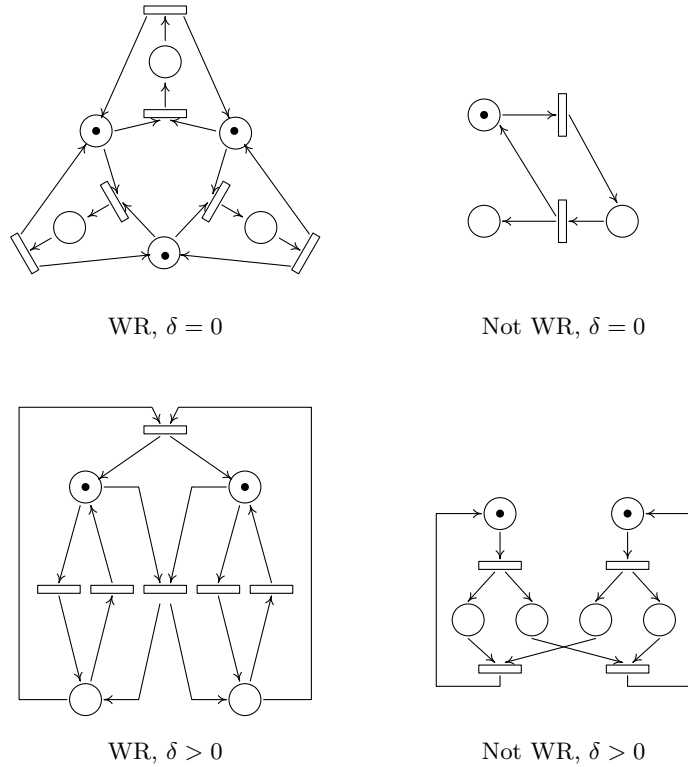
Fig. 3. Deficiency zero and weak reversibility are independent.
