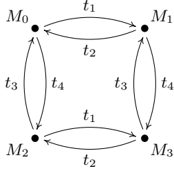
Fig. 2. Marking graph.
