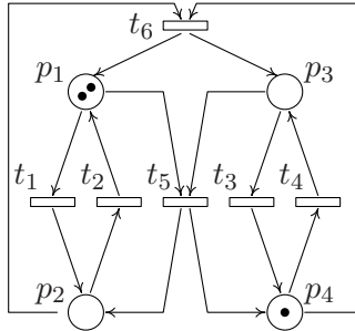
Figure 1: Petri net.
