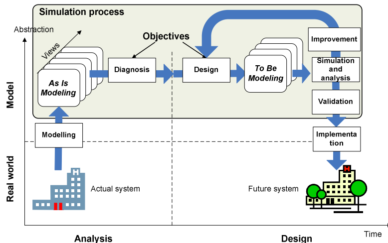
Figure 1: Reengineering methodology
