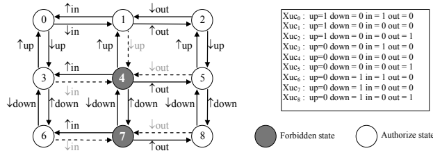
Figure 7. Prehensor Position automaton
