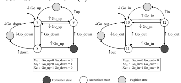
Figure 6. Cylinders output automata
