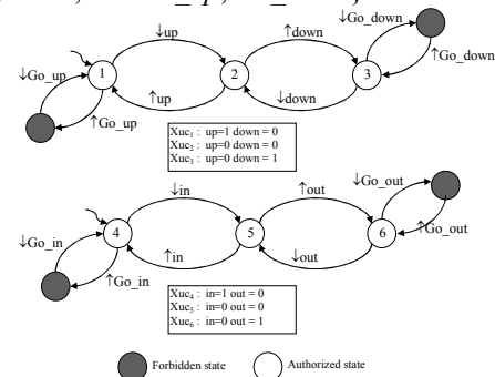
Figure 5. Cylinders position automata
