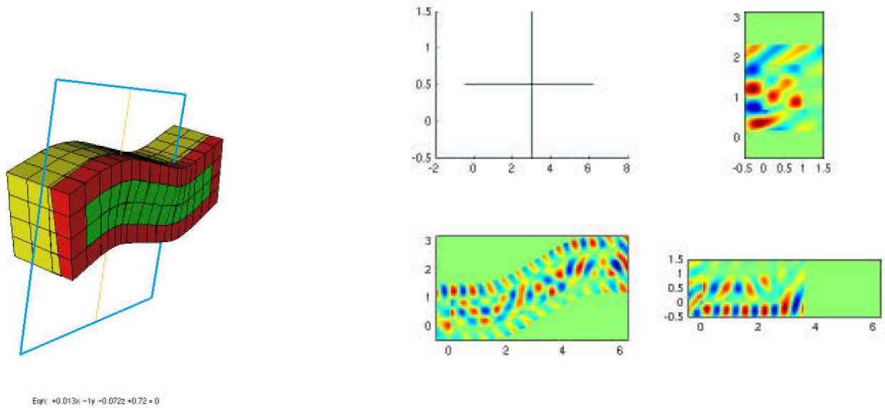
Fig. 18. At left mesh of the cavity, at right real part of x-component of electric field
